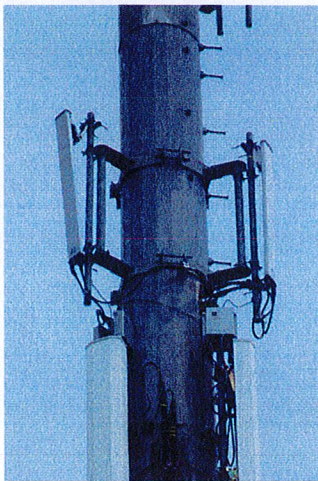
AT&T ARRAY TO BE REMOVED, SHOWN AT 75 FOOT LEVEL (2 nd from BOTTOM)
