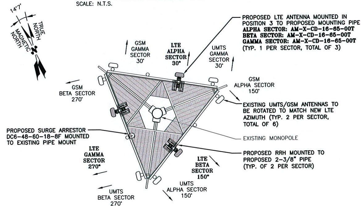
PROPOSED LTE ANTENNA PLAN
