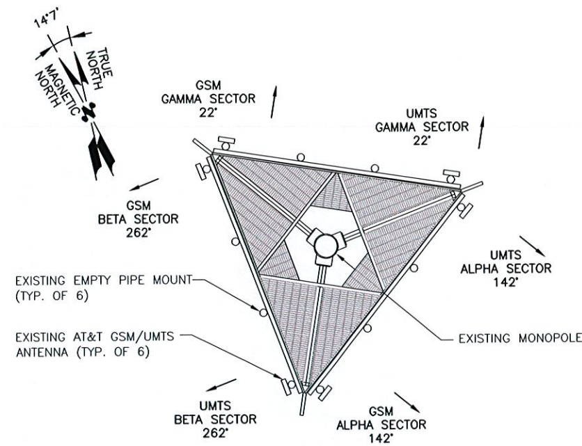
EXISTING GSM/UMTS ANTENNA PLAN
