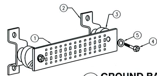
GROUND BAR - DETAIL
