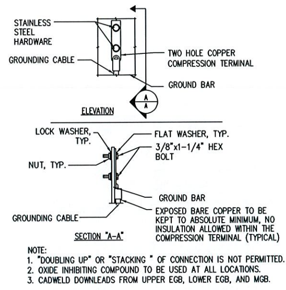
TYPICAL GROUND BAR CONNECTION DETAIL
