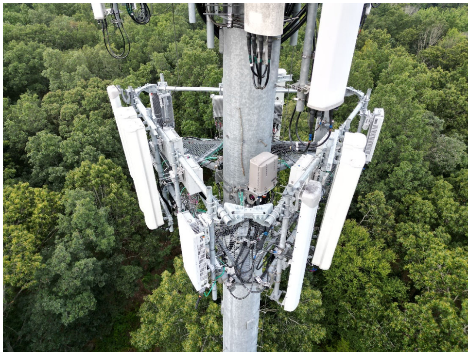
Fig. 2: Overall View of Antennas, RRHs & OVP
