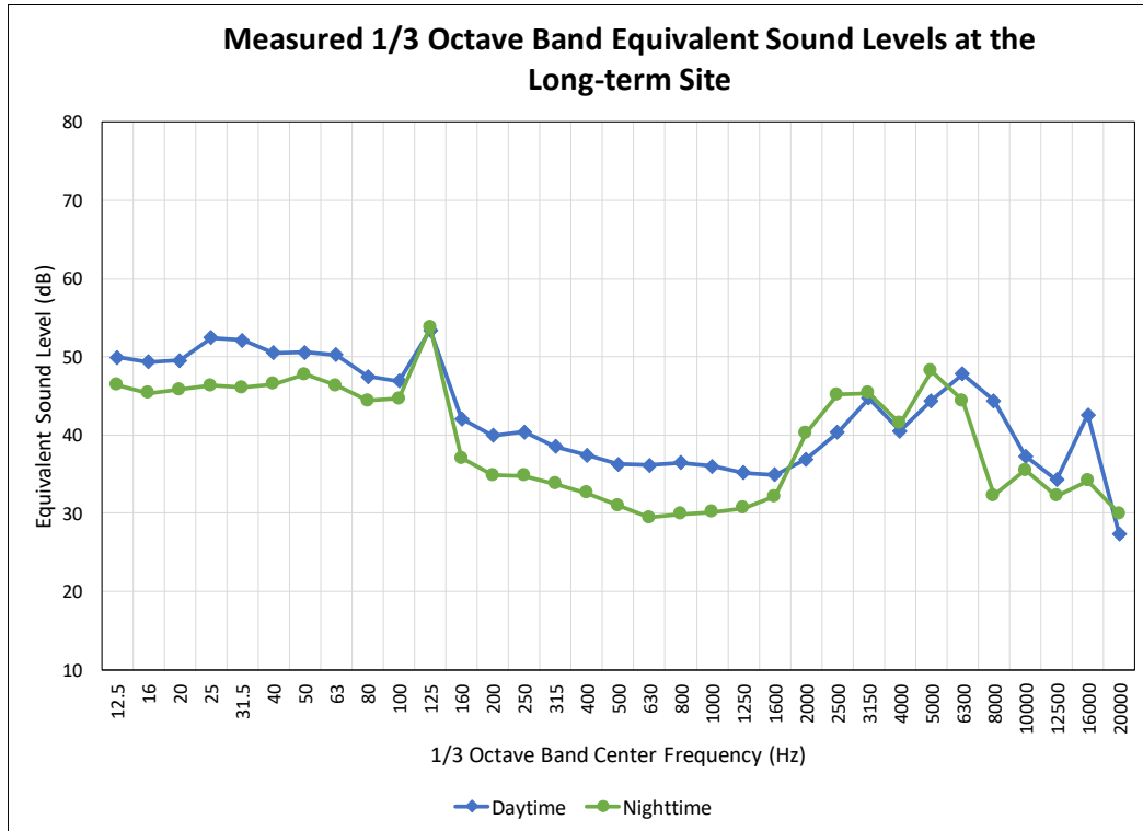
Figure 10. Measured Daytime and Nighttime Sound Level Spectra at the Long-term Site (Unfiltered)
