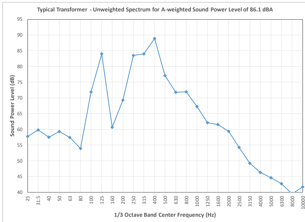
Figure 11. Typical Transformer Spectrum for an A-weighted Sound Power Level of 86.1 dBA
