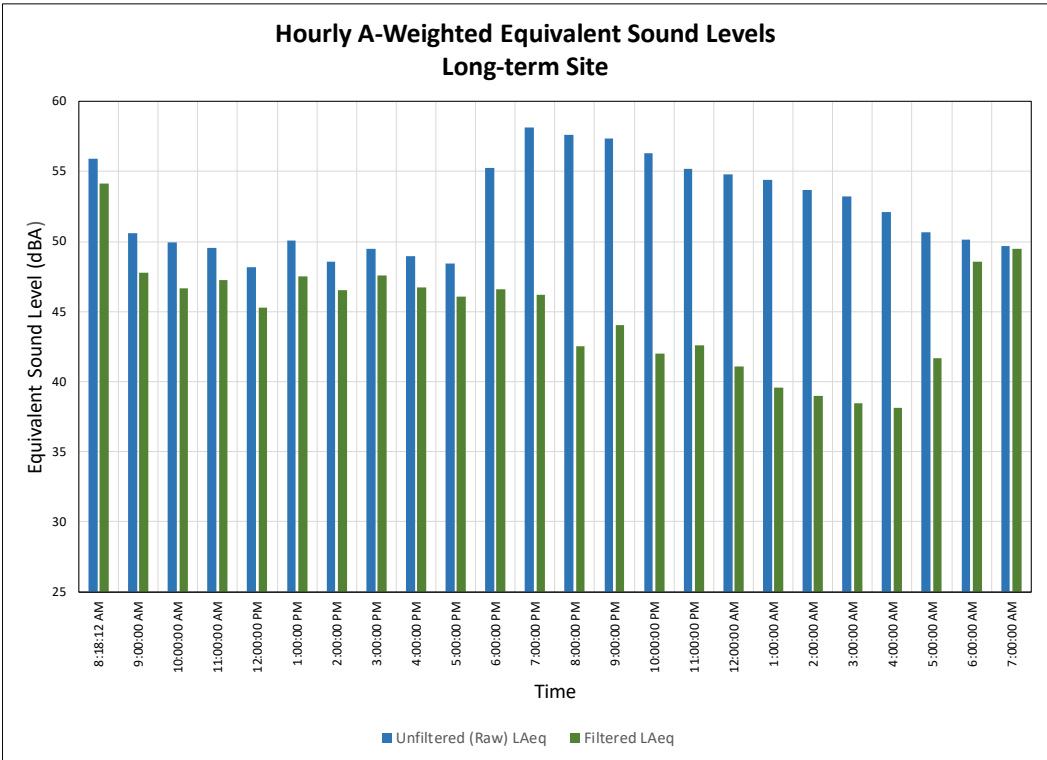
Figure 9. Hourly A-weighted Equivalent Sound Levels at Long-term Site (Unfiltered and Filtered)
