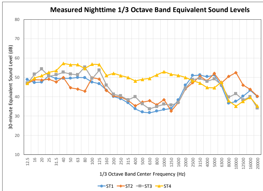
Figure 7. Measured Nighttime 1/3 Octave Band Sound Levels at the Short-term Sites (Unfiltered)
