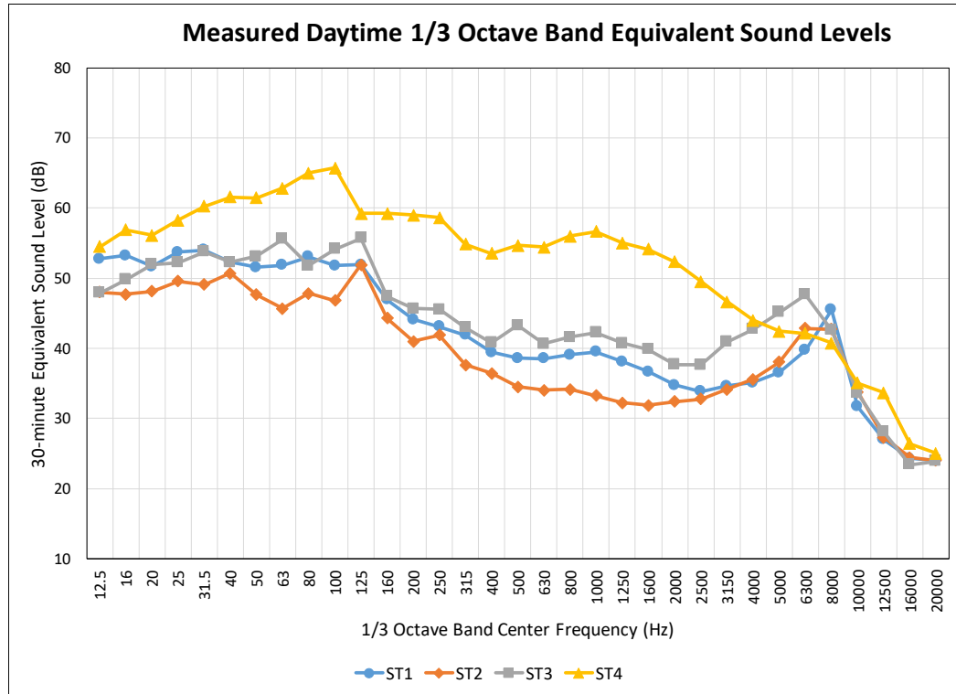
Figure 6. Measured Daytime 1/3 Octave Band Sound Levels at the Short-term Sites (Unfiltered)
