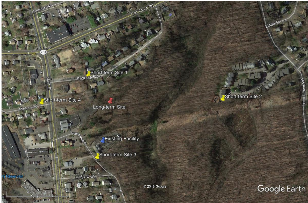
Figure 1. Preconstruction Noise Monitoring Sites from August 12 to 13, 2019
