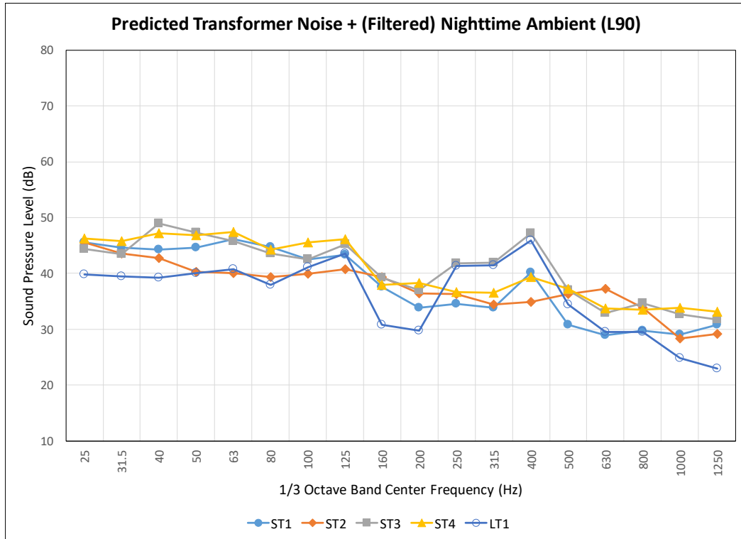
Figure 13. Predicted Transformer Noise Added to (Filtered) Nighttime Ambient L 90 in 1/3 Octave Bands at Measurement Sites
