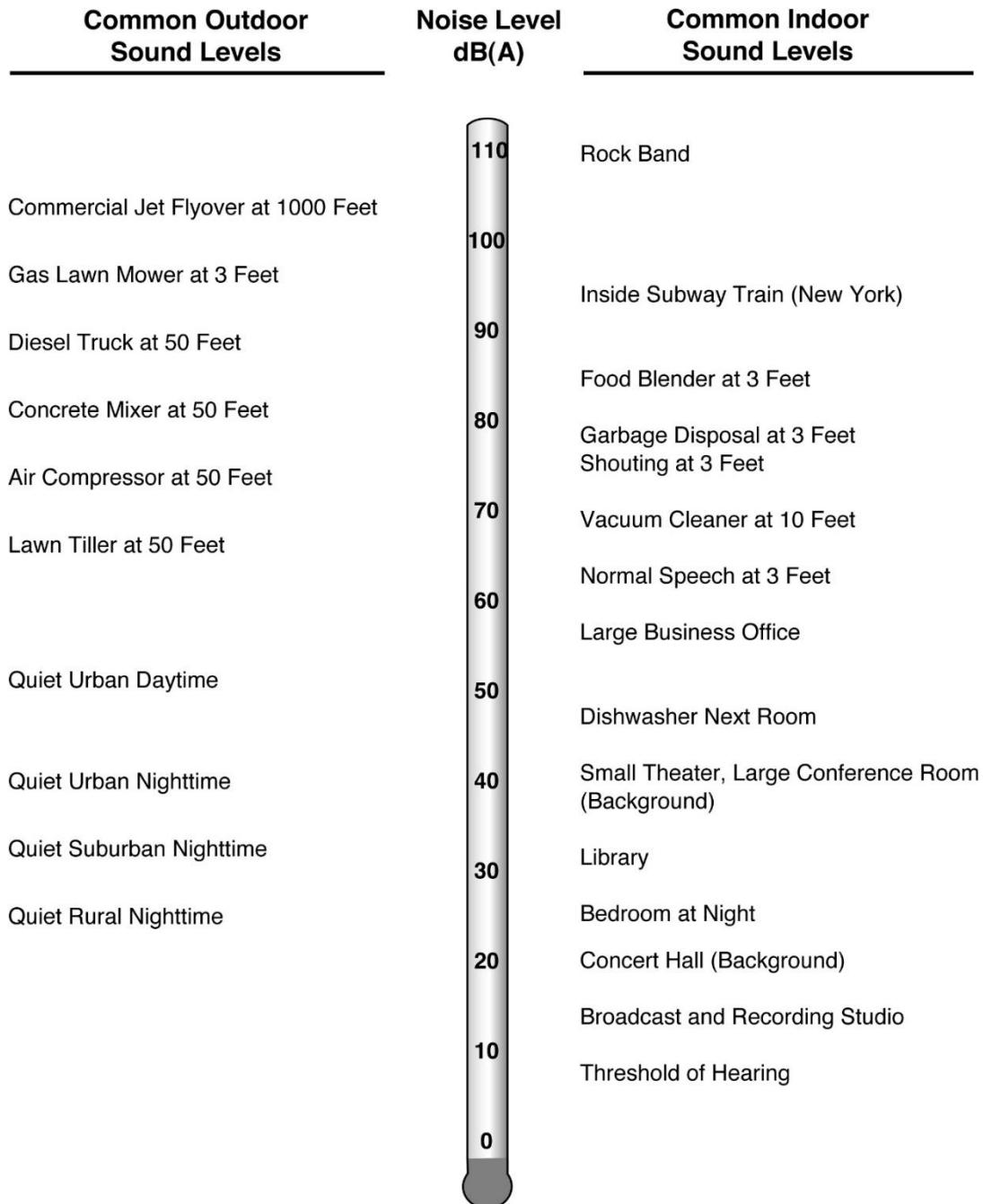
Figure B-2. Common Outdoor and Indoor A-weighted Sound Levels
