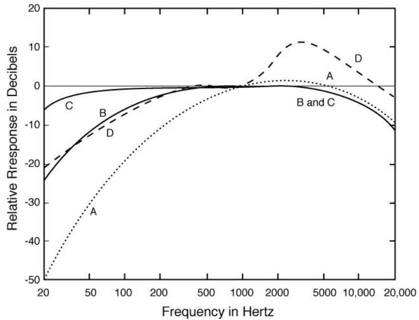
Figure B-1. Relative Response of A-, B-, C-, and D-Weighting Networks
