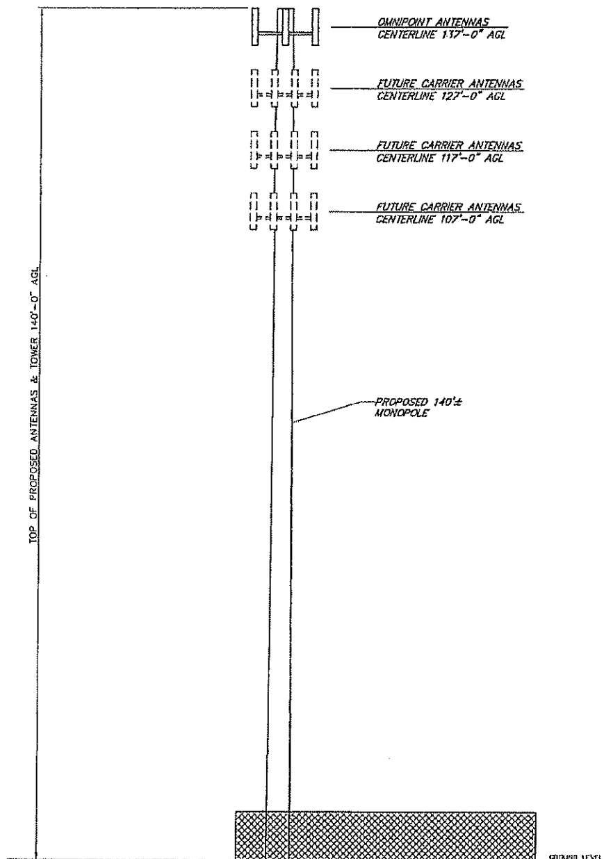
1 TOWER ELEVATION SCALE: 1" = 20' 0 10 20 SCALE IN FEET
