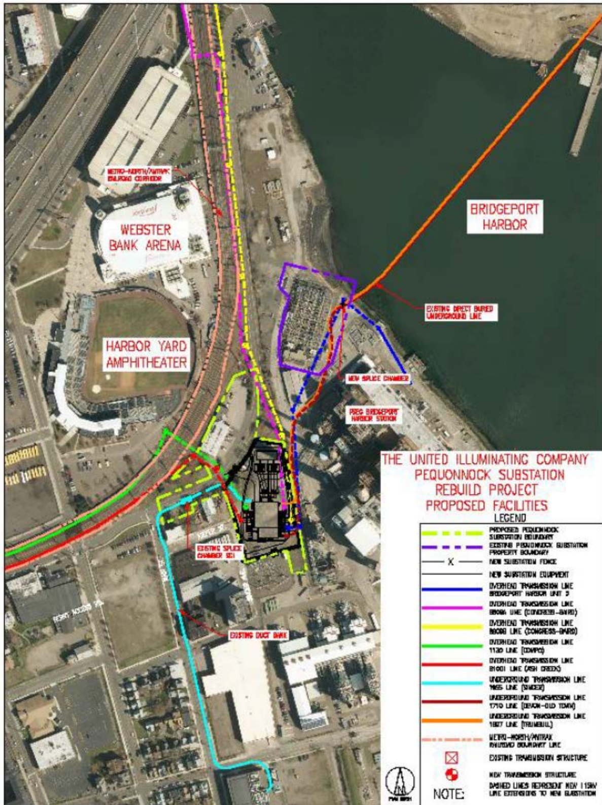
Replacement Substation Site Plan
