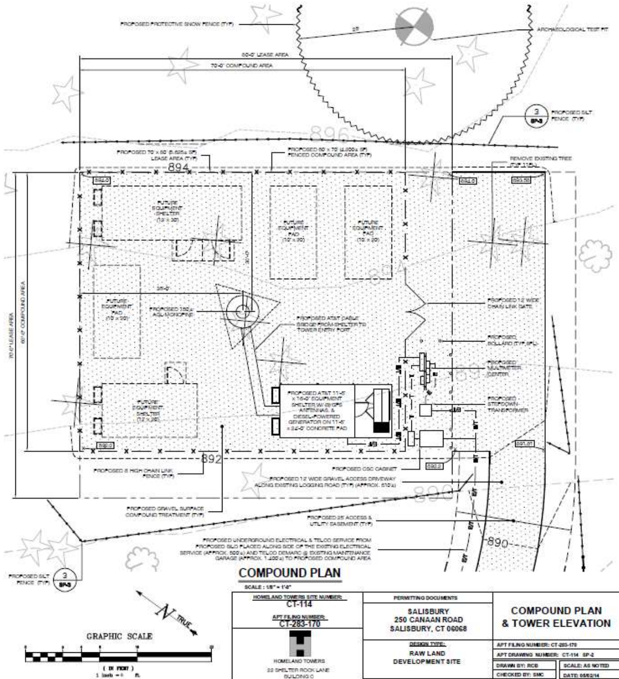
Figure 2 – Compound Plan (at Revised Location)
