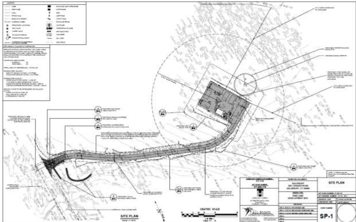
Figure 3 – Access Drive Drawing (at Revised Location)
