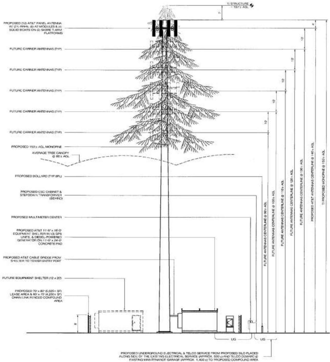
Figure 4 – Tower Elevation Drawing (at Revised Location)
