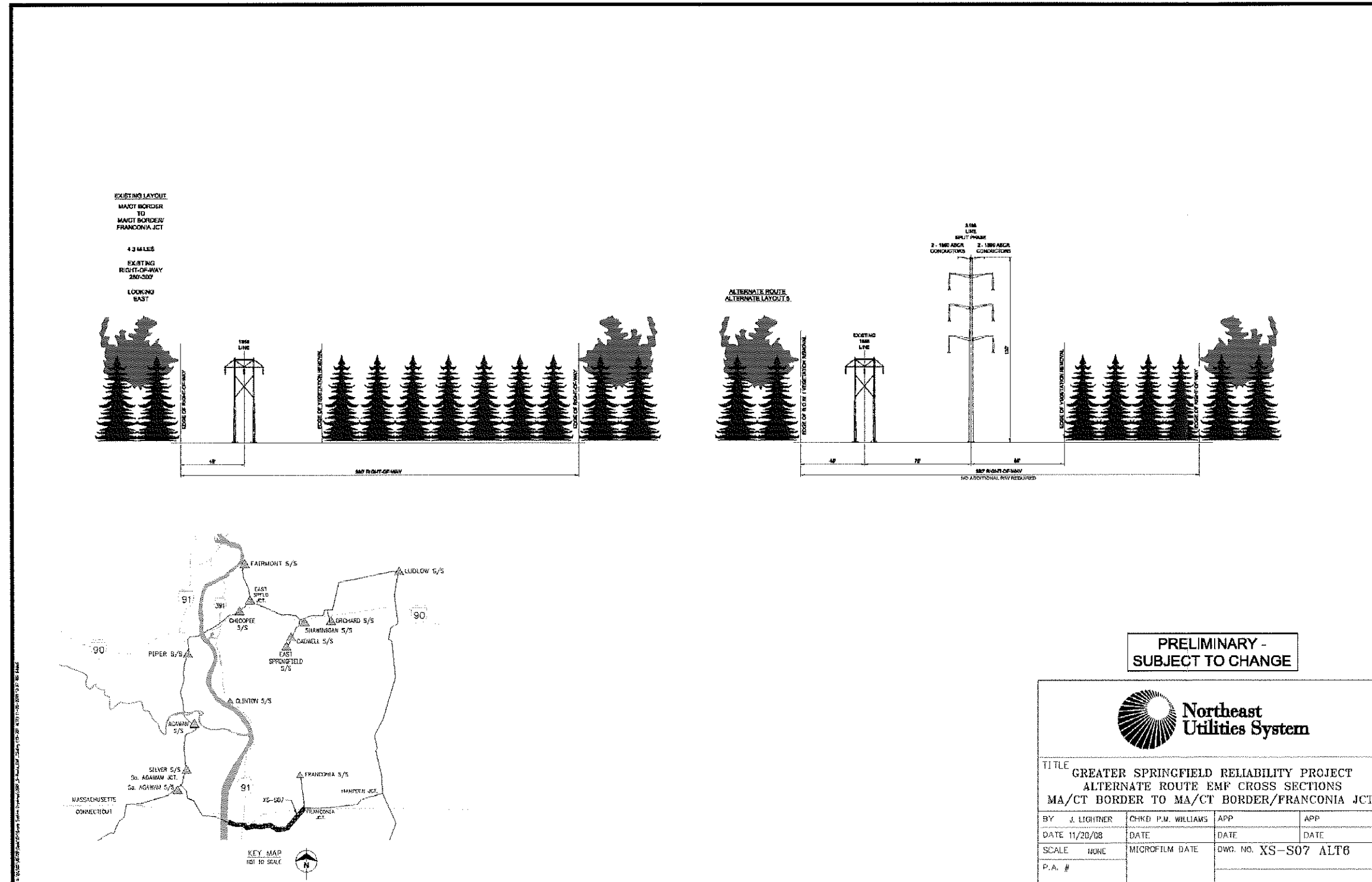
Figure 15: XS-S07 Cross Section, Alternate Configuration 6
