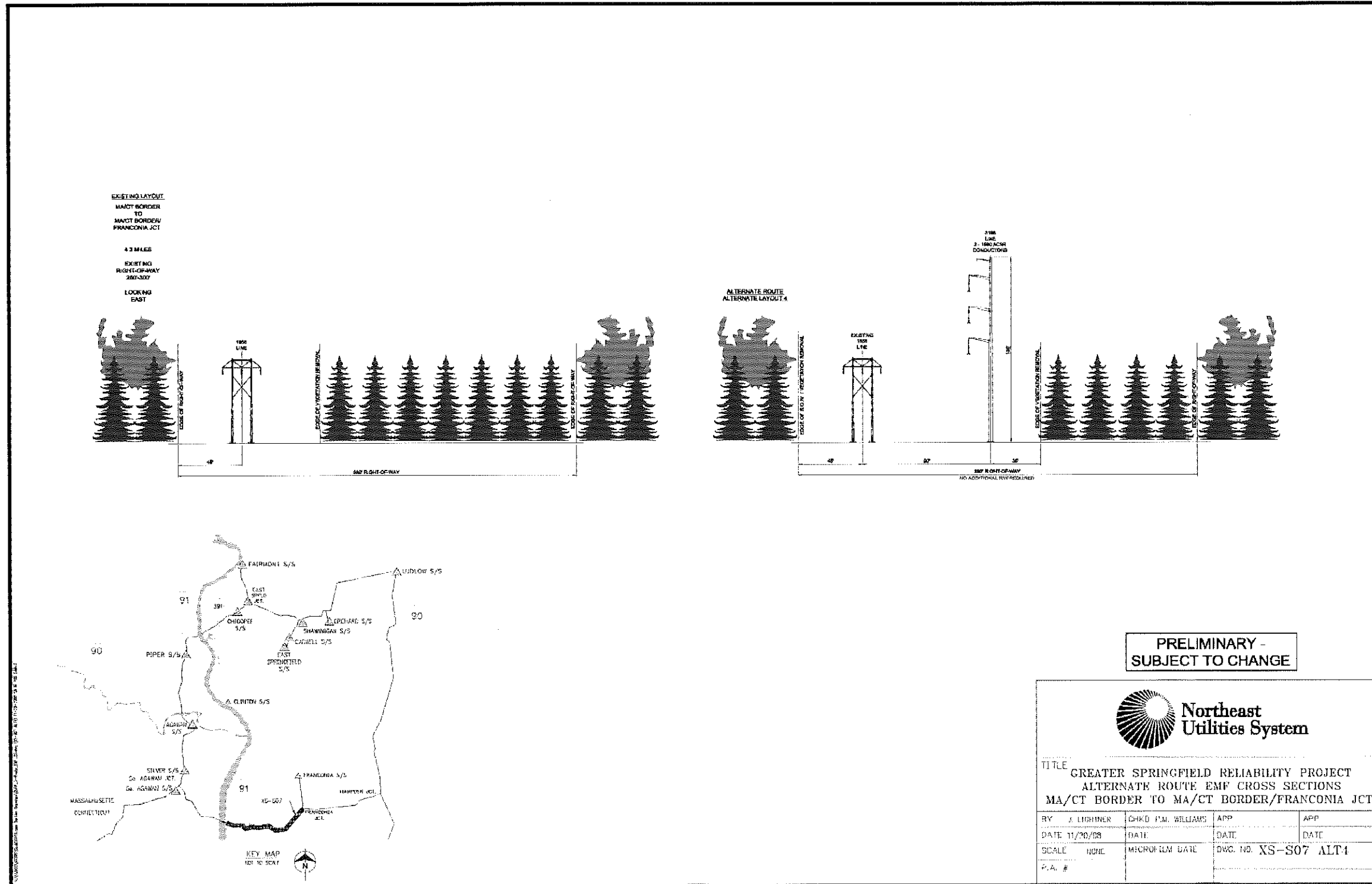
Figure 13: XS-S07 Cross Section, Alternate Configuration 4
