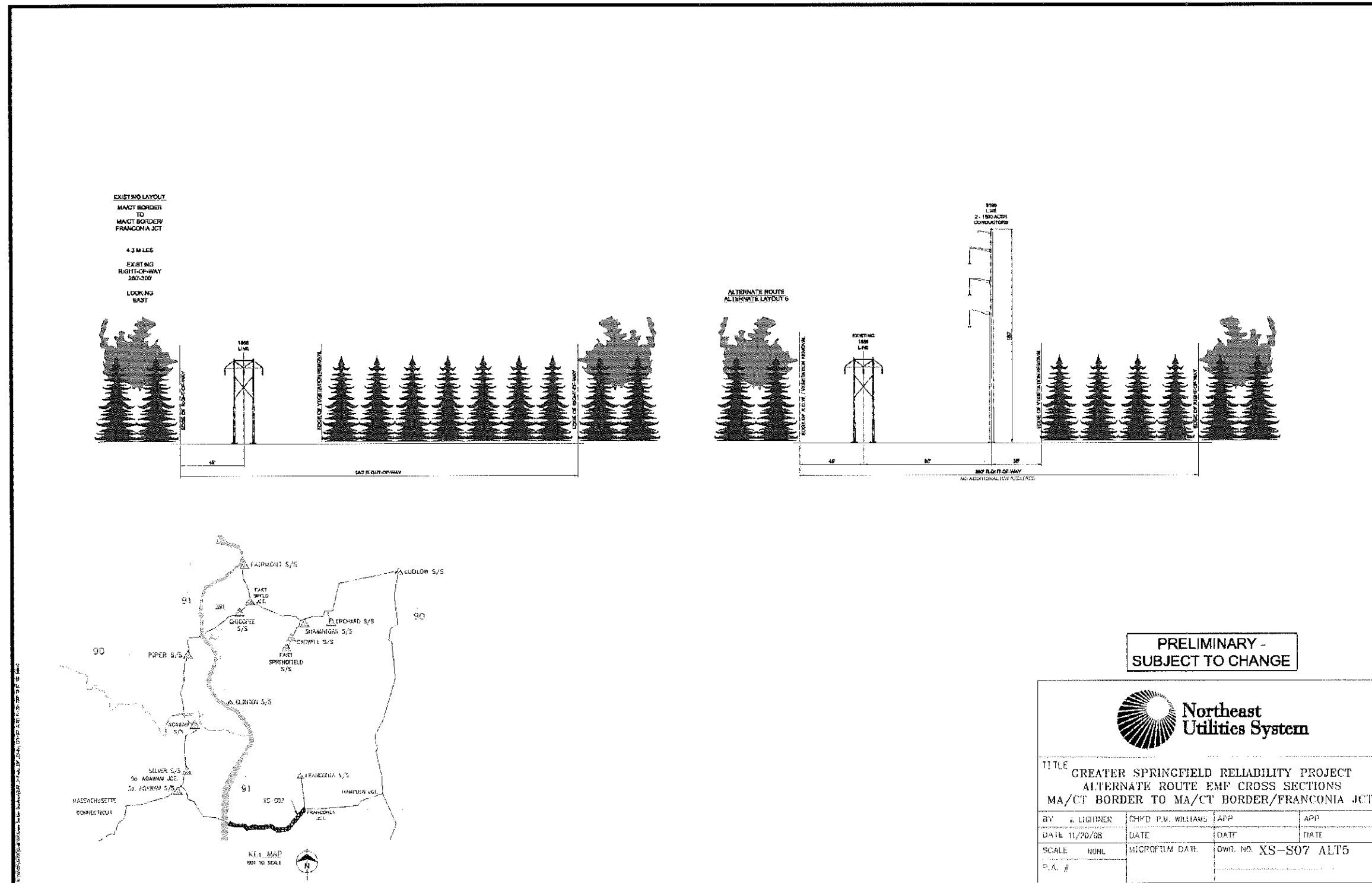
Figure 14: XS-S07 Cross Section, Alternate Configuration 5
