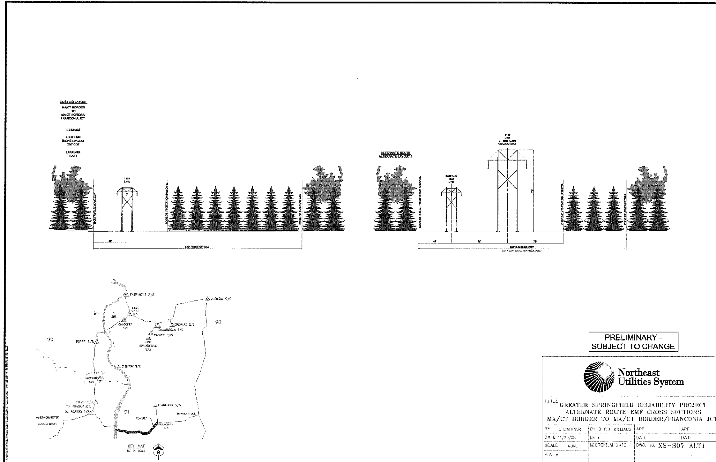
Figure 10: XS-S07 Cross Section, Alternate Configuration 1
