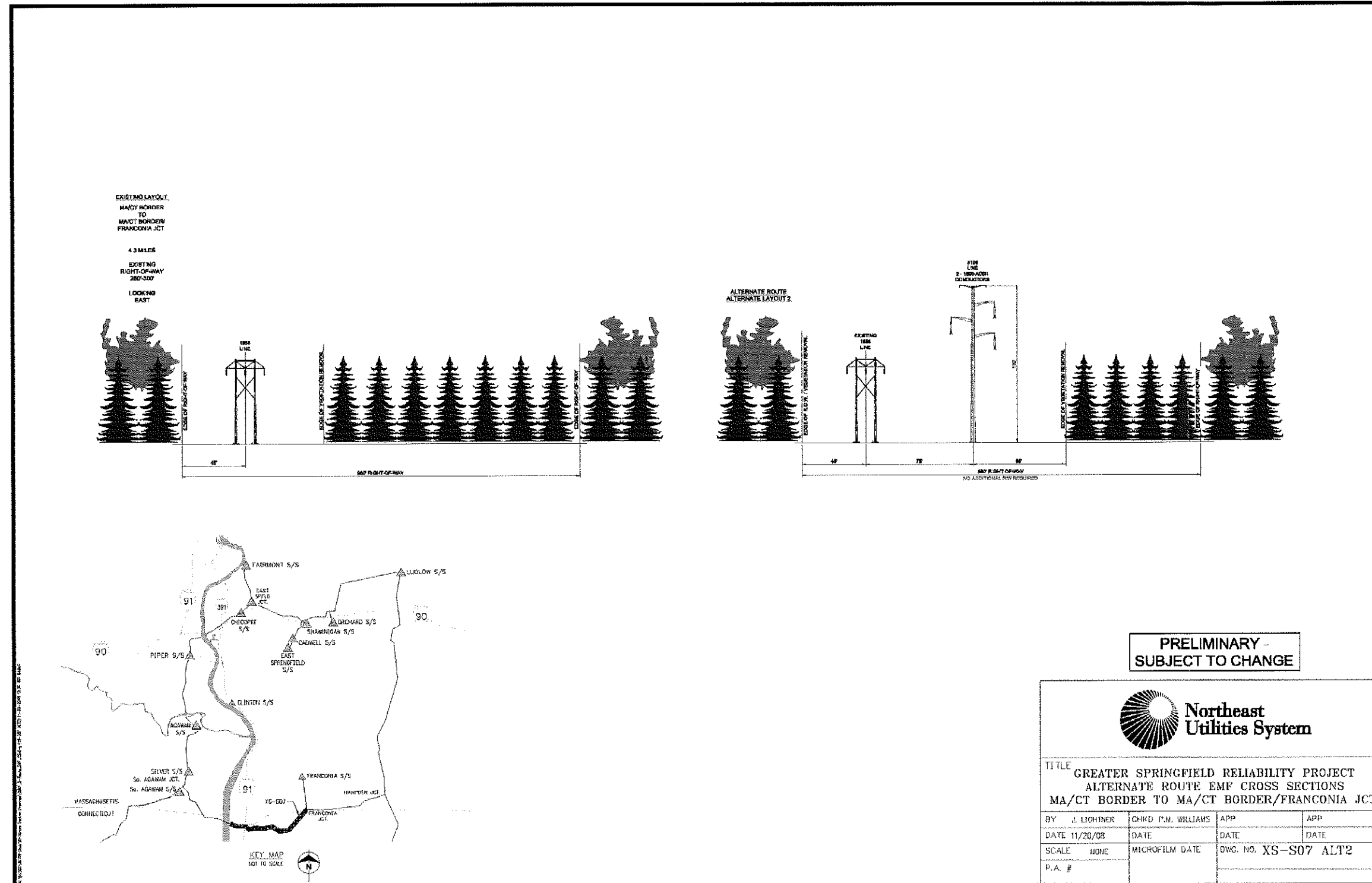
Figure 11: XS-S07 Cross Section, Alternate Configuration 2
