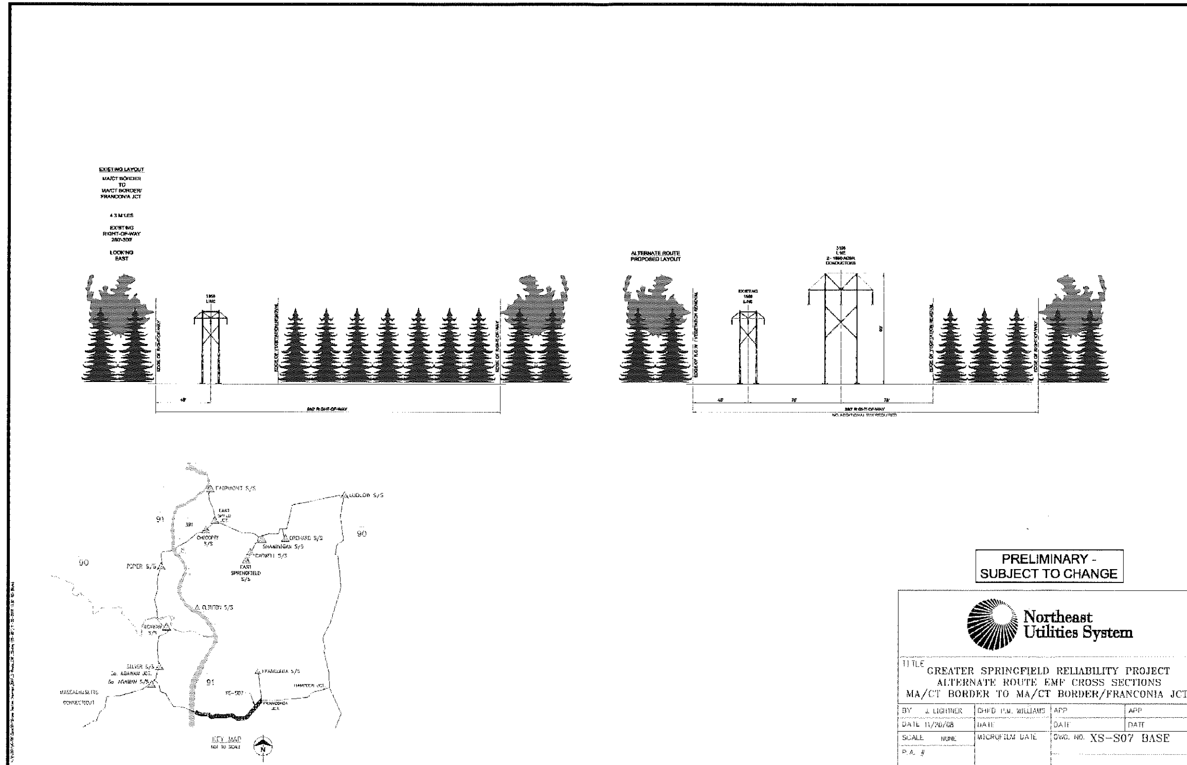
Figure 9: XS-S07 Cross Section, Base Configuration
