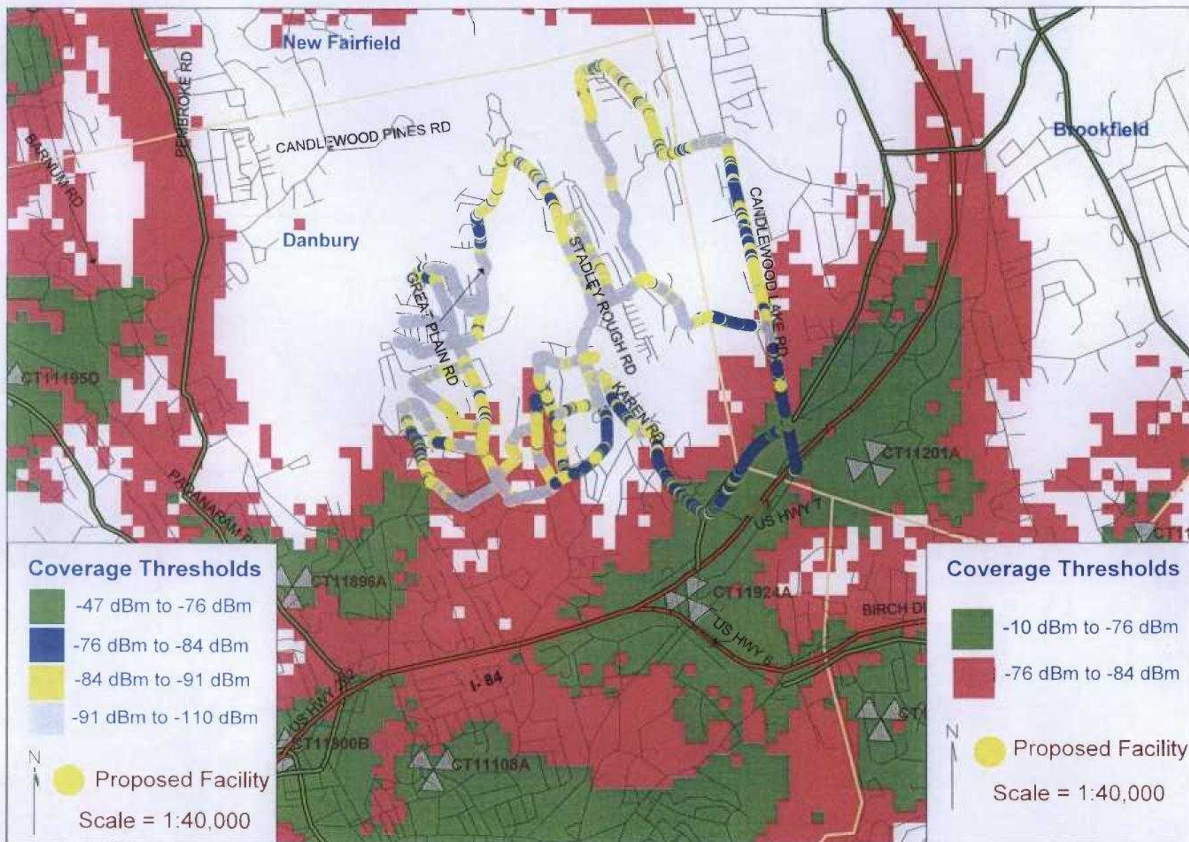
Existing Coverage With Drive Test Results - Active Call: Taken August 20, 2008
