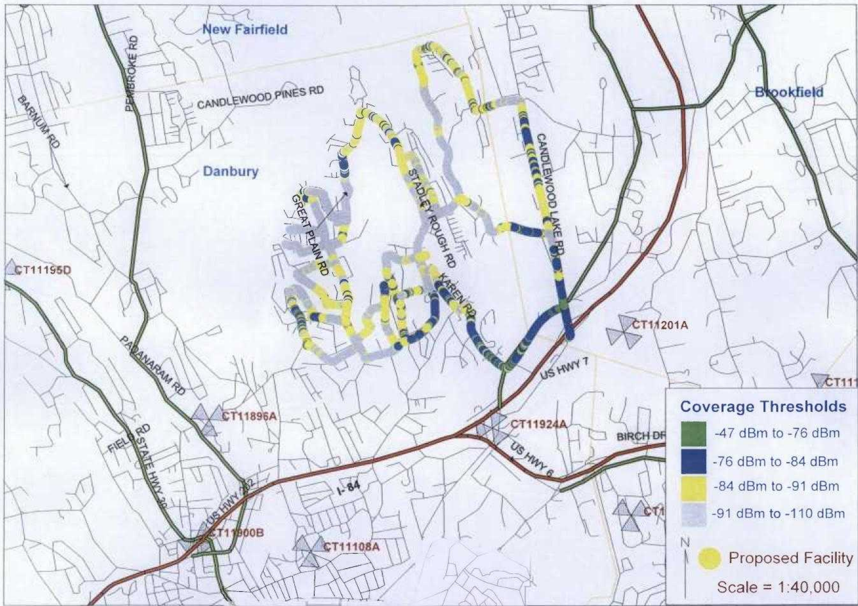
Drive Test Results - Active Call: Taken August 20, 2008
