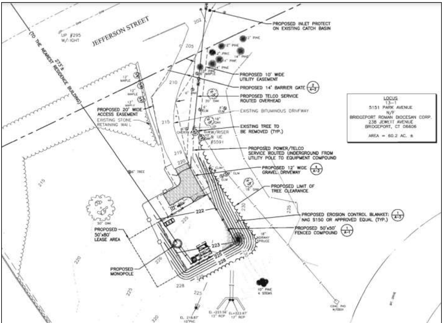
Figure 2: Site Plan
