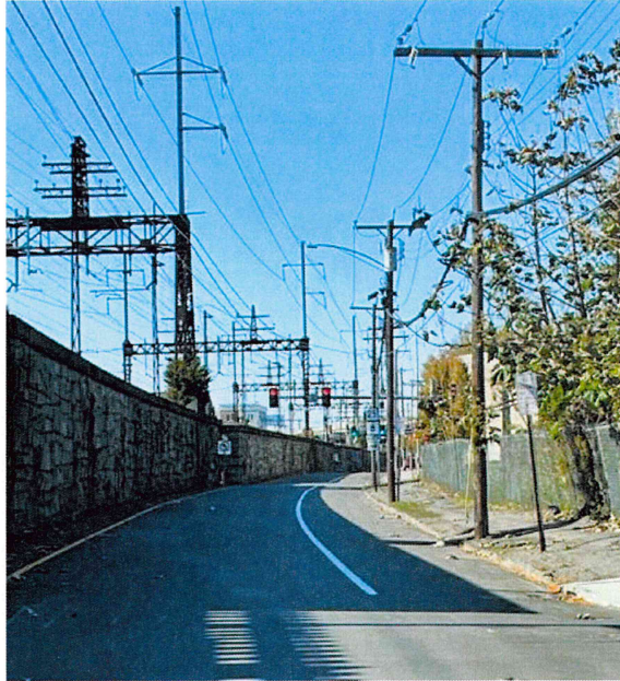
Figure 16. Underground cable route with easy road access. Distribution line (right) could be installed in the duct system.
