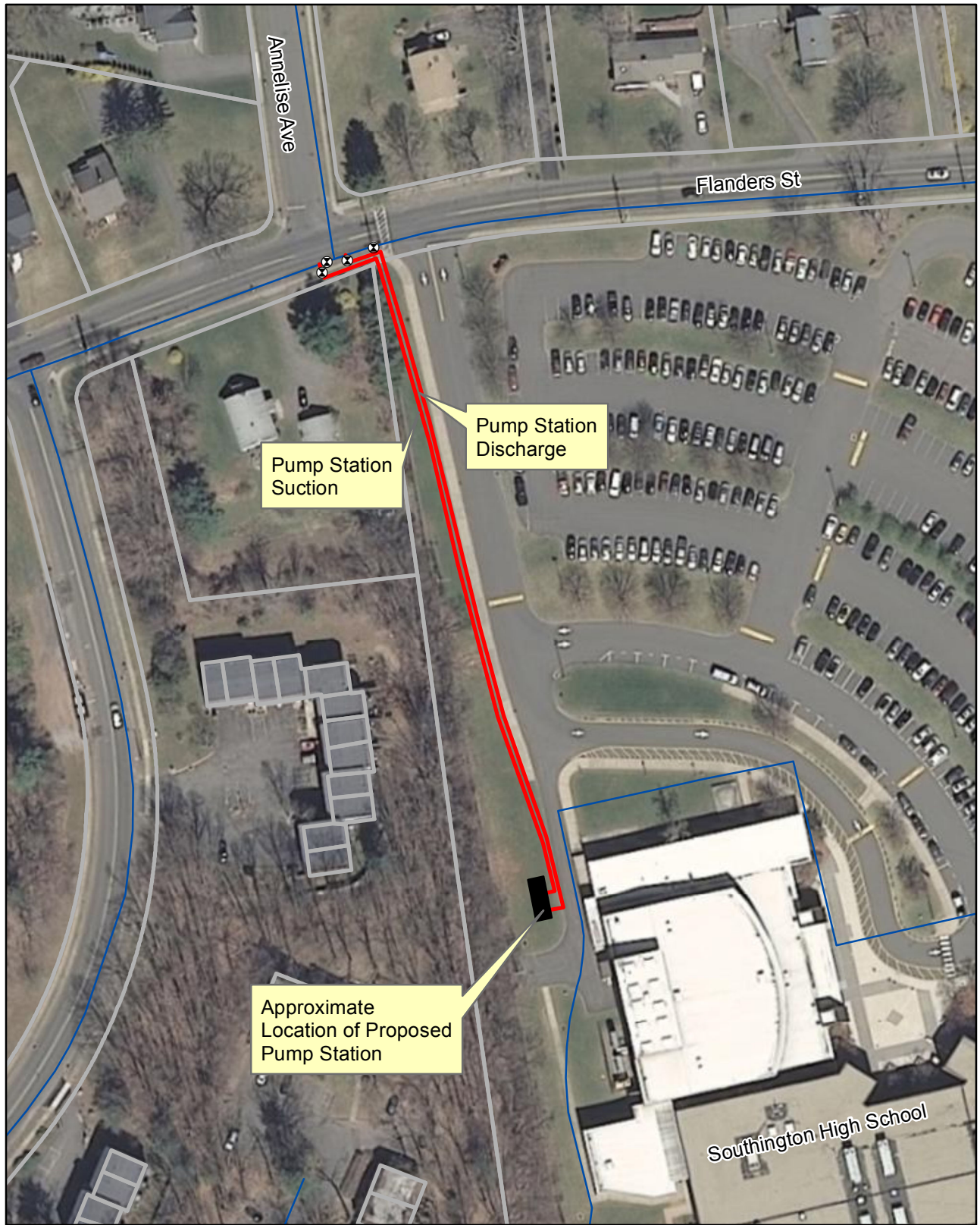
Figure 3 Proposed Pump Station
