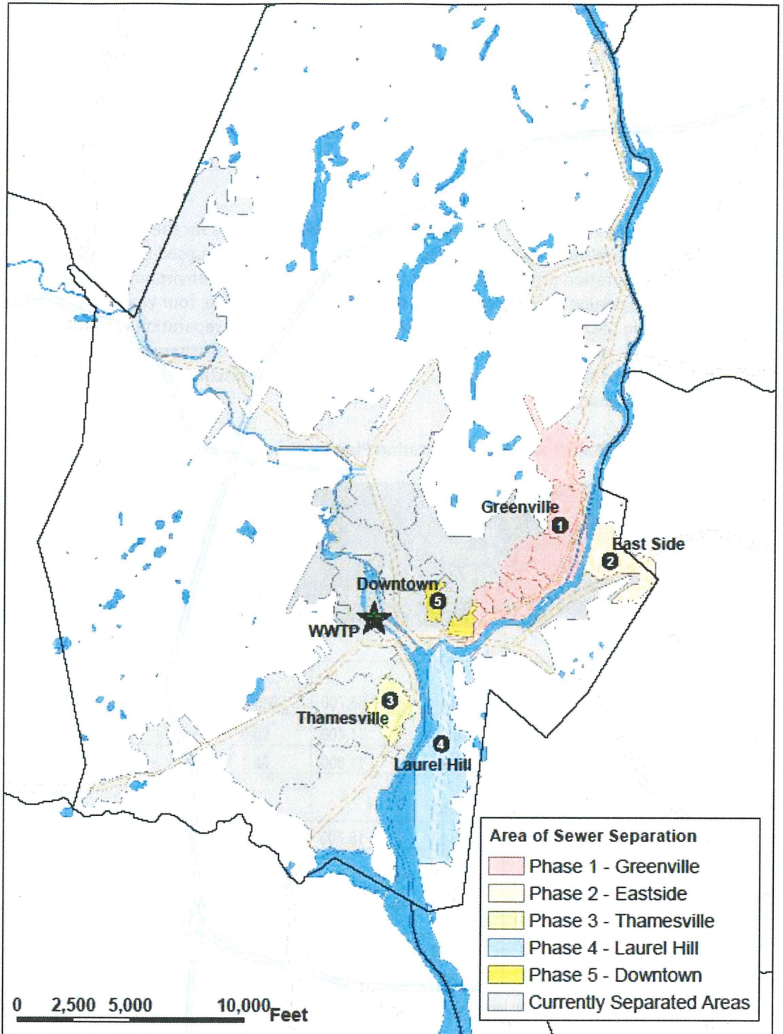
Figure 2 – Recommended Five-Phase Plan for Complete Sewer Separation in Norwich
