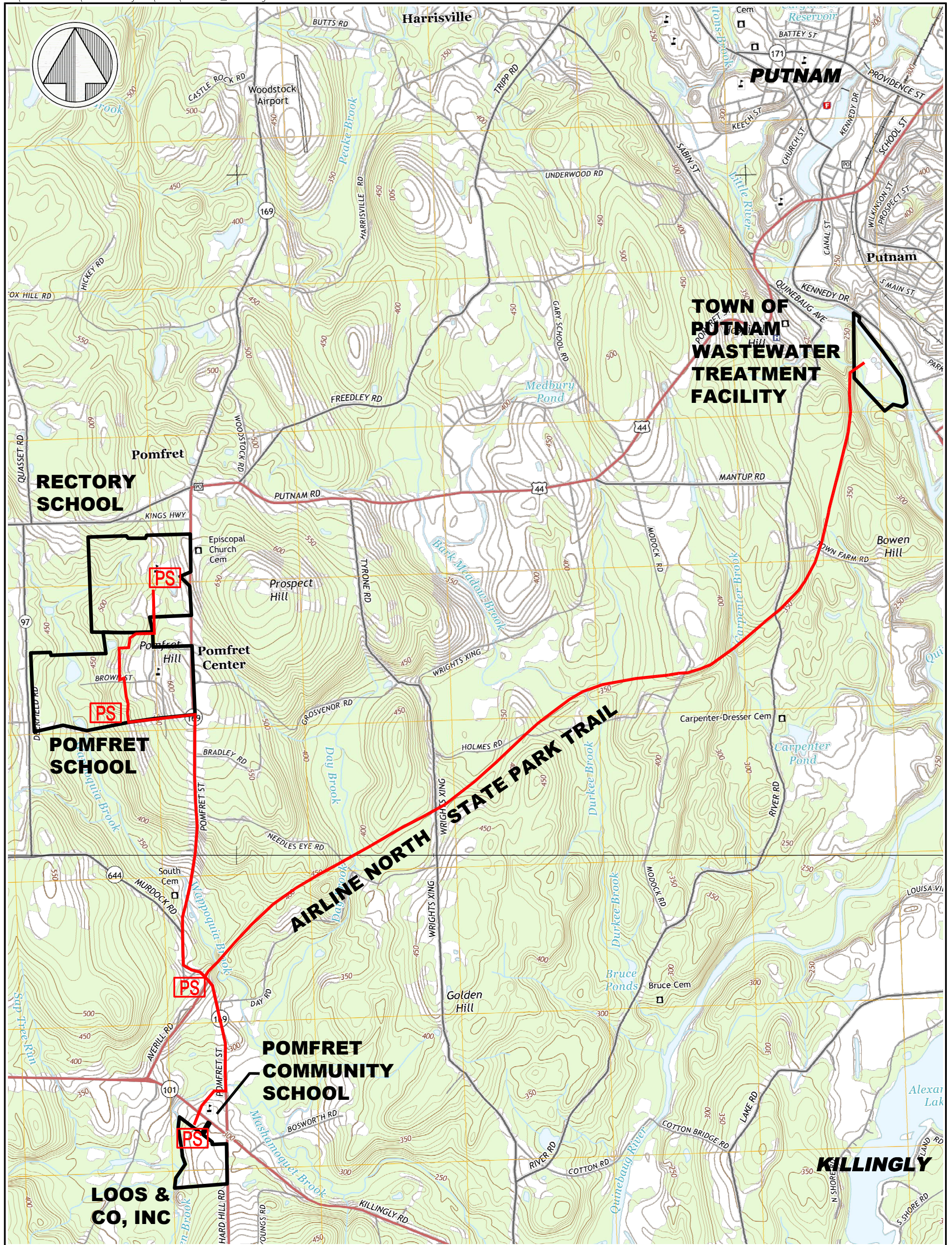
FIGURE 12 OPTION 3C - CONNECT TO PUTNAM POTW VIA AIRLINE NORTH STATE PARK TRAIL POMFRET, CONNECTICUT JULY 2015 SCALE: 1"=2000'
