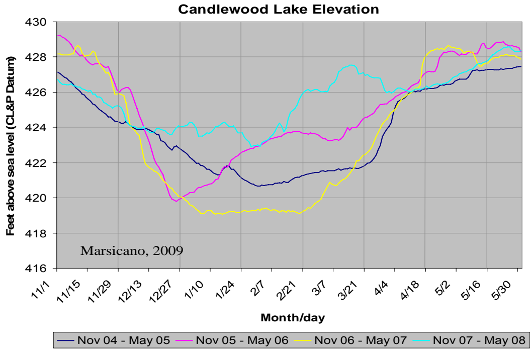
Figure 3. Depth and duration of drawdown from 2004 -2008 in Lake Candlewood.
