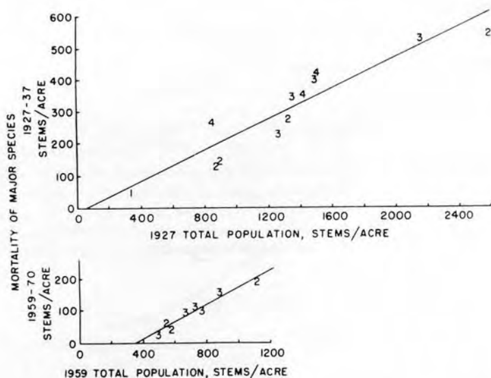
Figure 2. Periodic mortality of major species in tracts without major defoliation. The numbers are the sites: muck (1), medium moist (3) and dry (4). The line is the straight line that best fits the observations. Upper. Meshomasic series, 1927-37. Lower. Natchaug, Norfolk and Catlin Wood of the New series, 1959-70.
