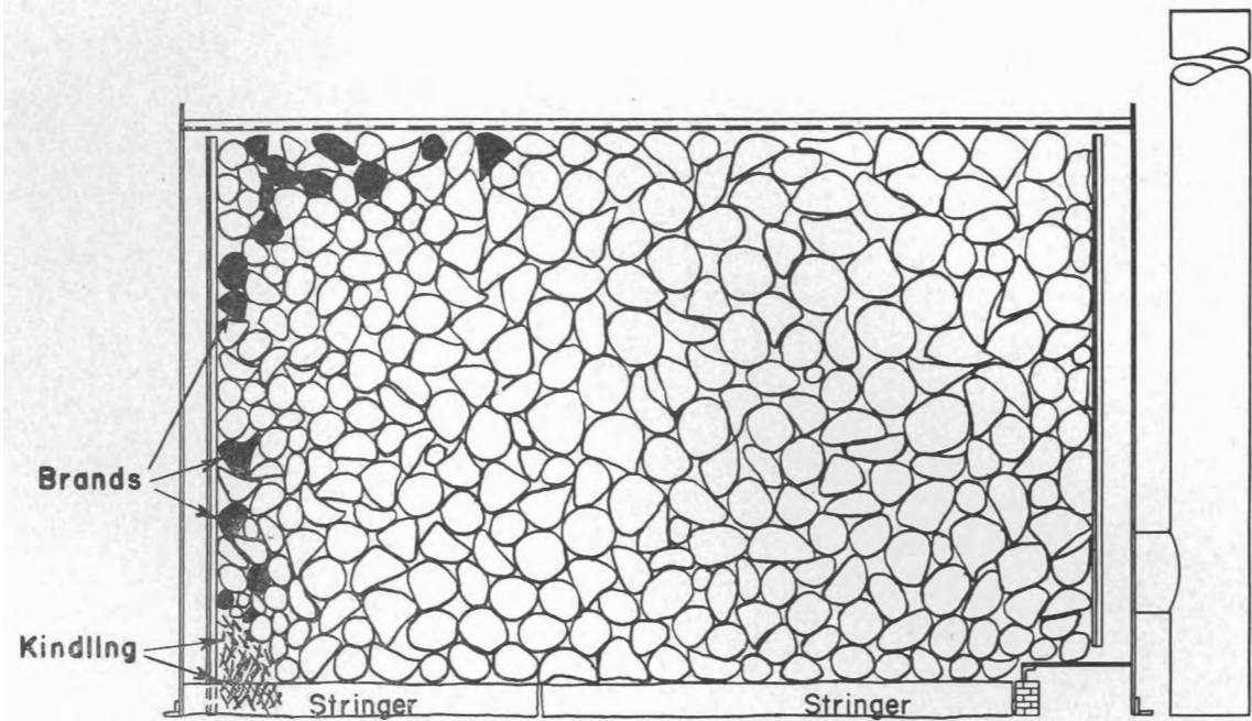
FIGURE 2. Vertical section through the one cord kiln showing the method of loading with wood.
