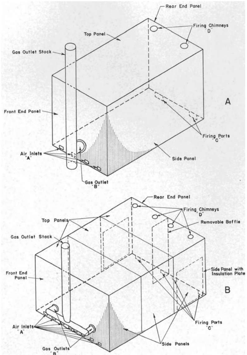
FIGURE 3. General View of the kilns showing relative position of the panels, firing ports, firing chimneys, gas outlets, air inlets, and gas outlet stack. A. One cord kiln. B. Four cord kiln.
