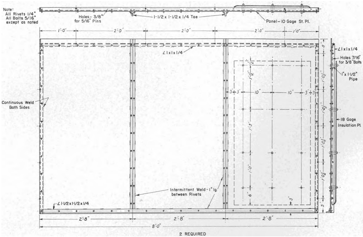
FIGURE 7. One cord kiln. Side panel.
