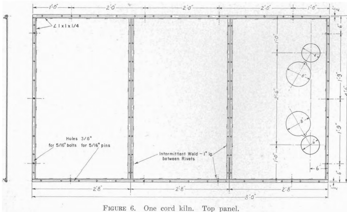
FIGURE 6. One cord kiln. Top panel.
