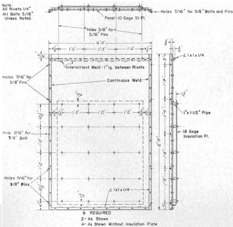
FIGURE 11. Four cord kiln. Side panel.
