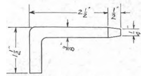
DETAIL OF PIN Use—Holding Panels in Place
