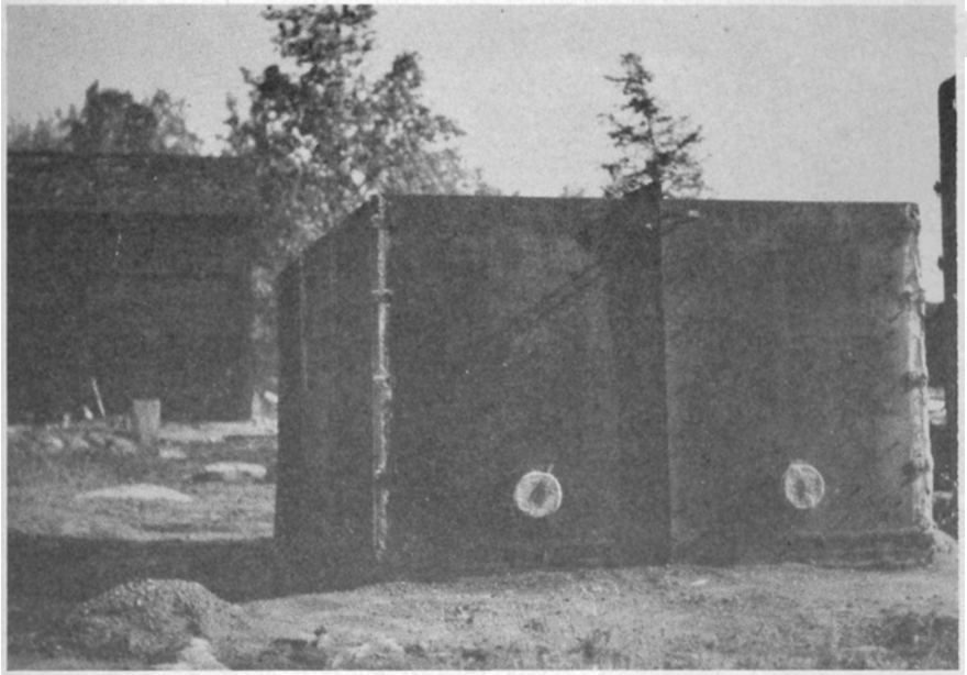
PLATE A. Front view of the four cord kiln with gas outlet stack removed.
