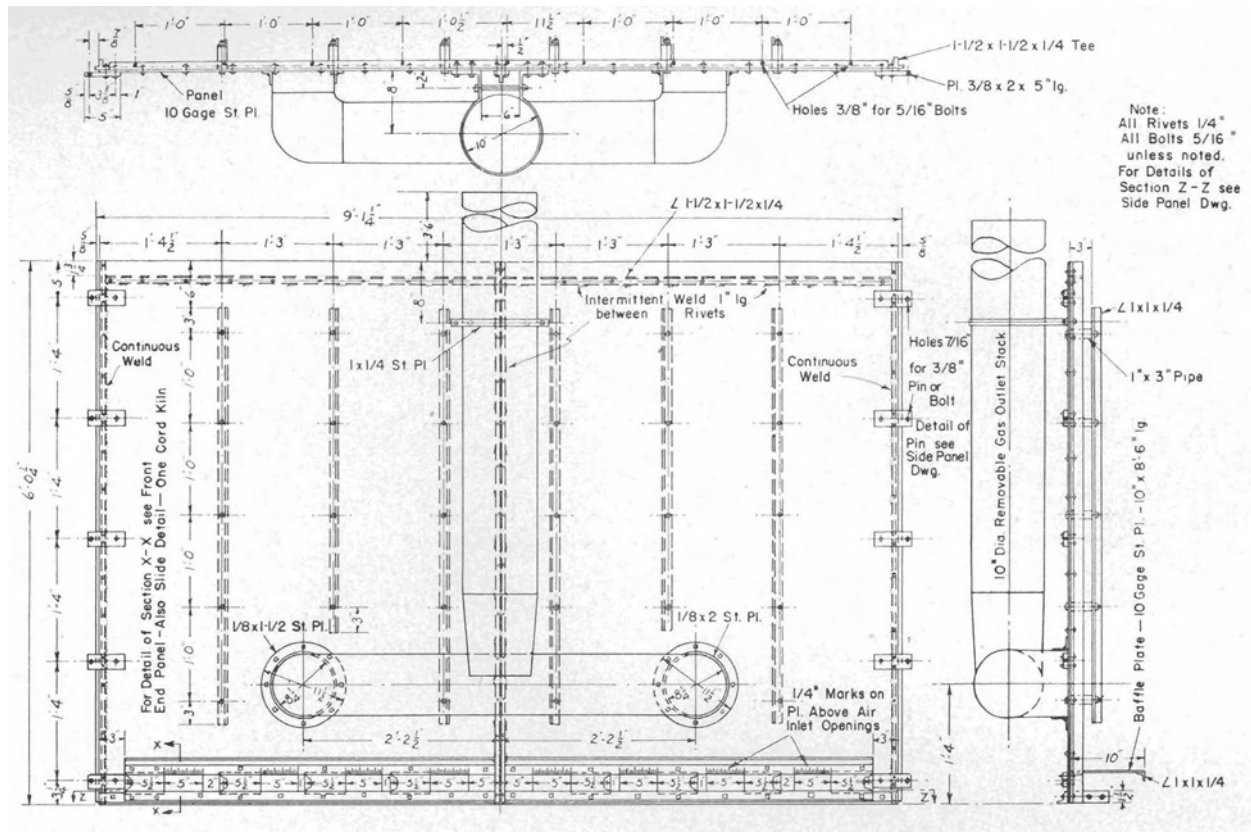
FIGURE 9. Four cord kiln. Front end panel and gas outlet stack. For details of air inlet slide construction, see Figure 4.
