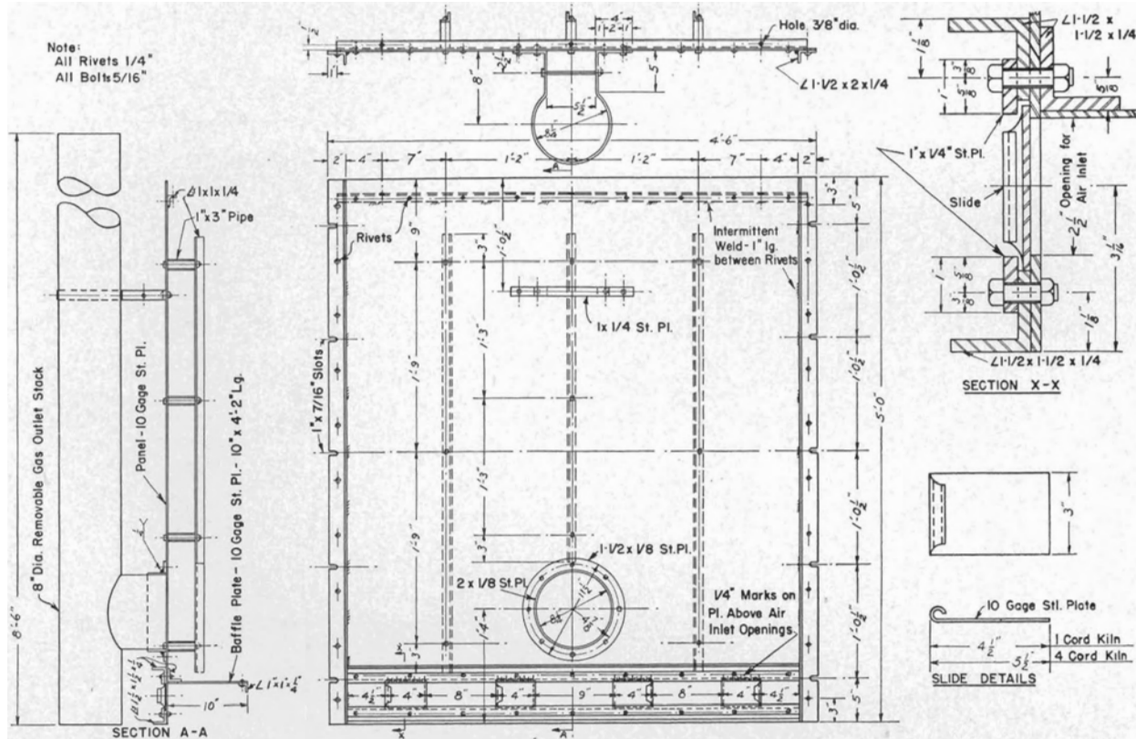
FIGURE 4. One cord kiln. Front end panel, gas outlet stack and details of air inlet slide construction.
