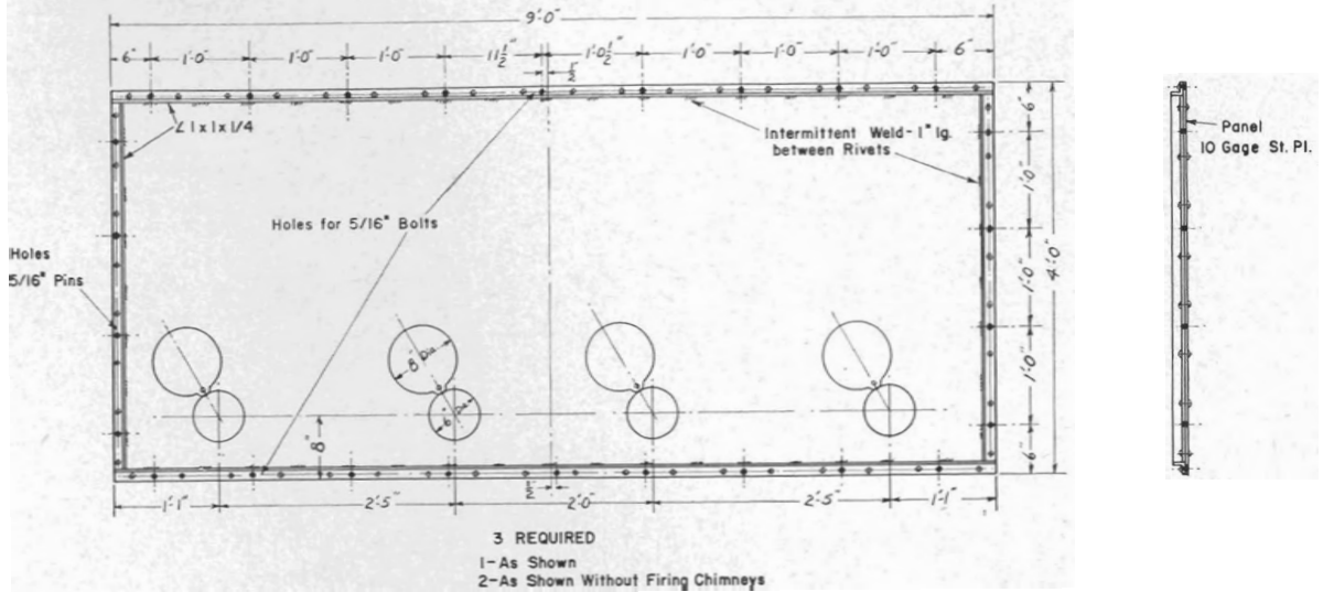
FIGURE 12. Four cord kiln. Top panel.
