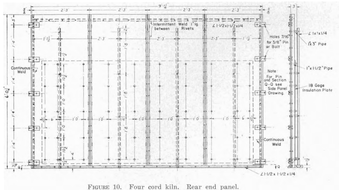
FIGURE 10. Four cord kiln. Rear end panel.
