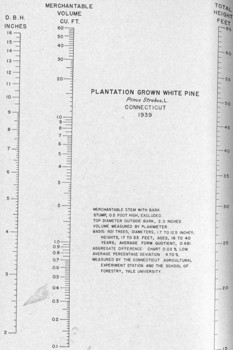
Chart II. Alinement chart for volumes of plantation grown white pine showing merchantable contents of the stem, including bark, in cubic feet.
