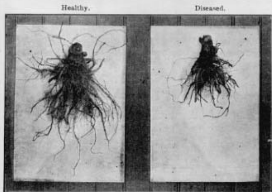
Fig. 11. Effect of rot on roots of mature field plants.
