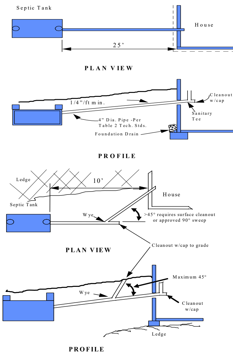
Figure 1 - Building Sewers
