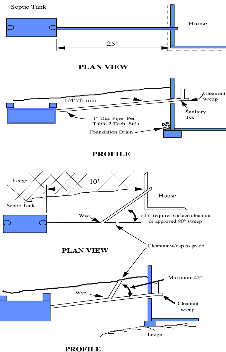
Figure 1 - Building Sewers
