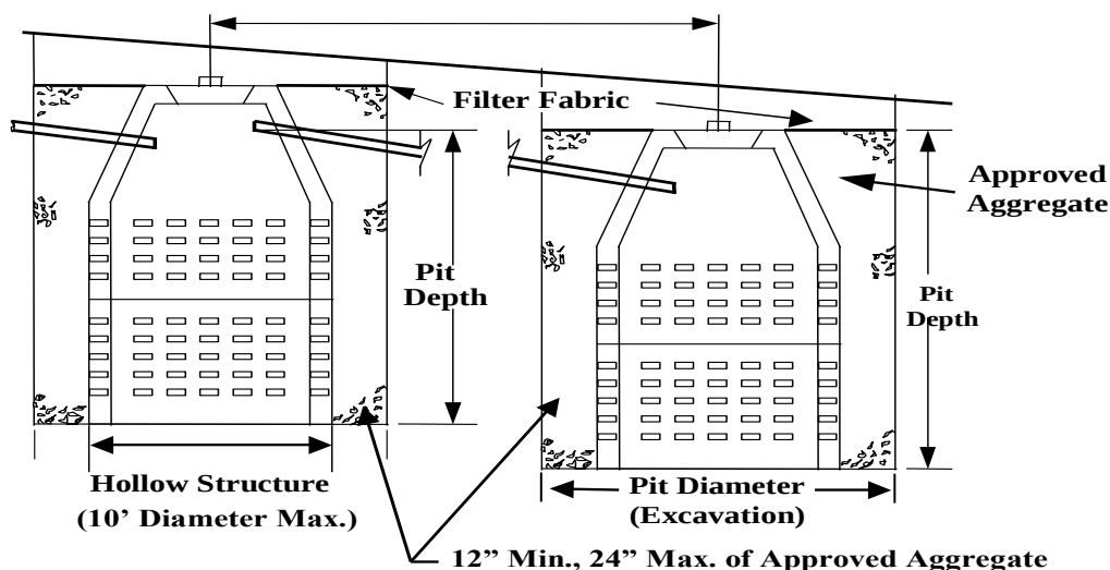
Figure 15 Leaching Pits
