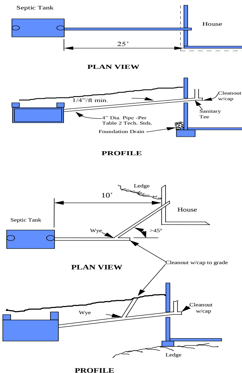
Figure 1 - Building Sewers
