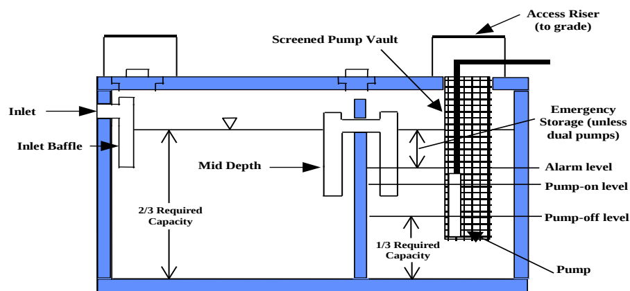
Figure 12 - Combination Septic Tank/Pump System with Tee Baffle Connection
