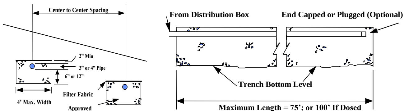
Figure 14 - Leaching Trenches
