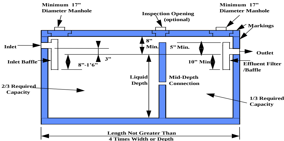
Figure 4 – Typical Septic Tank
