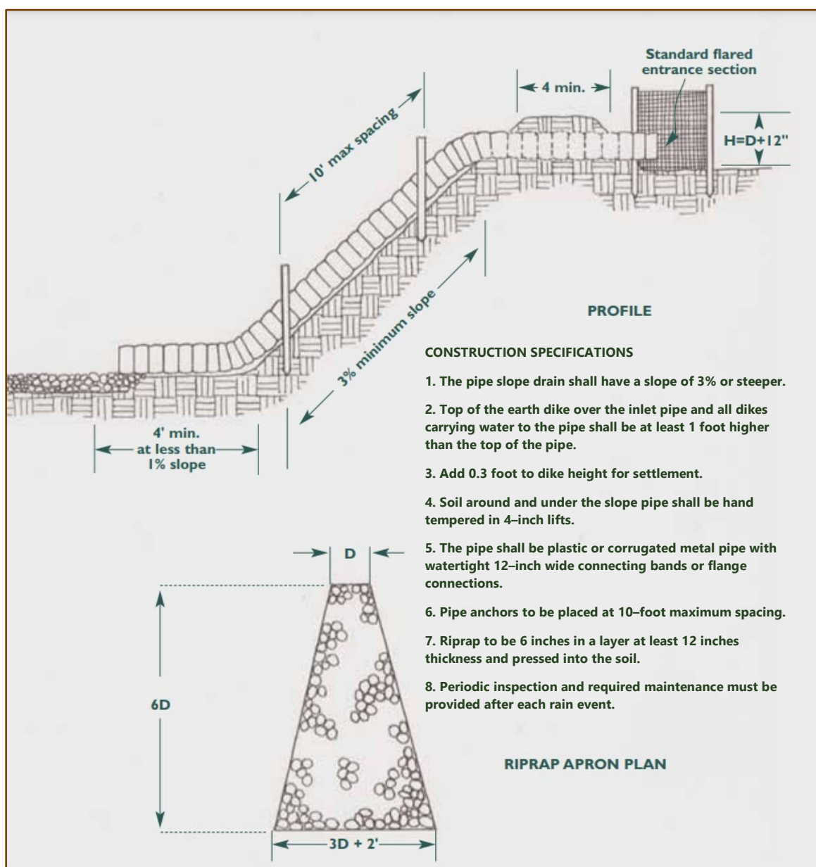
Figure 5-27 Example of Temporary Pipe Slope Drain
