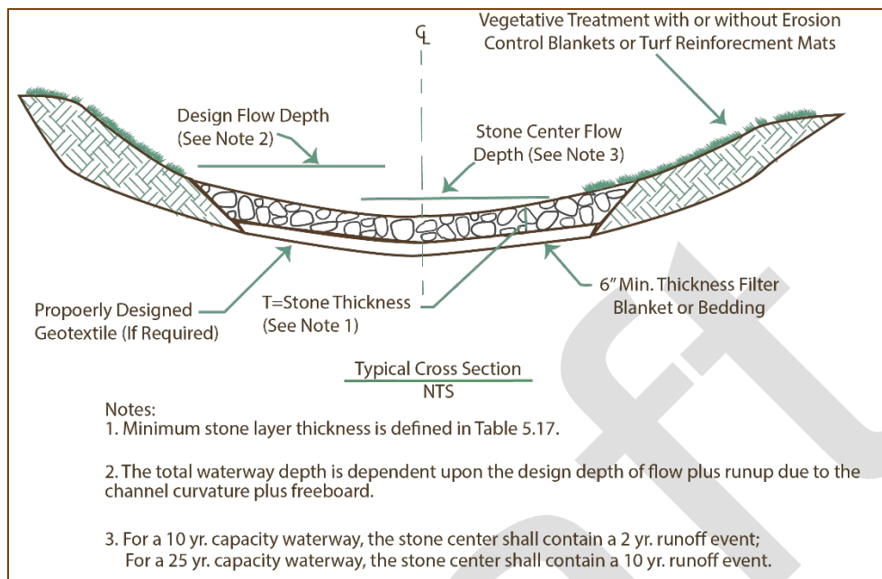
Figure 5- 42 Waterways with Stone Centers
