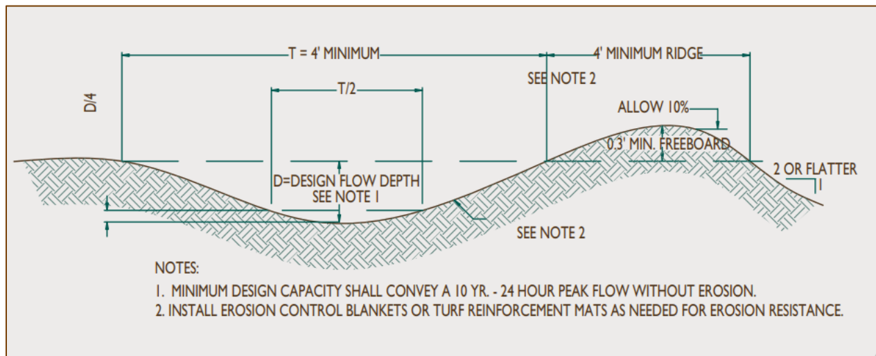
Figure 5- 51 Permanent Diversion
