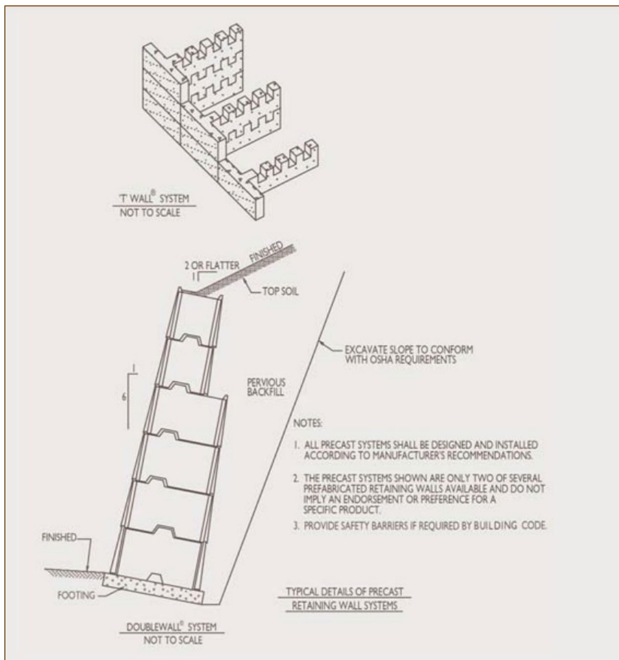
Figure 5- 16 Precast Retaining Walls
