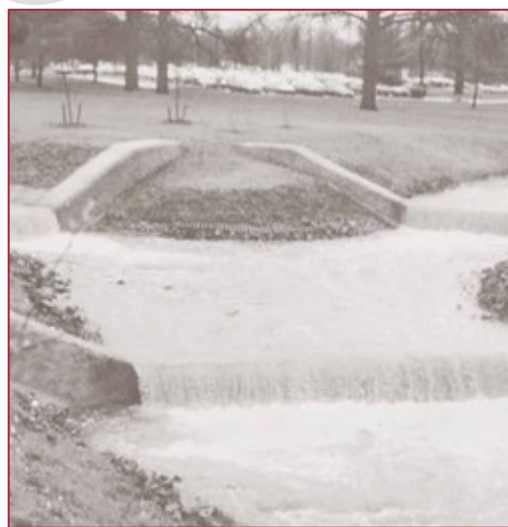
Figure 5- 24 Example of a Grade Stabilization Structure
