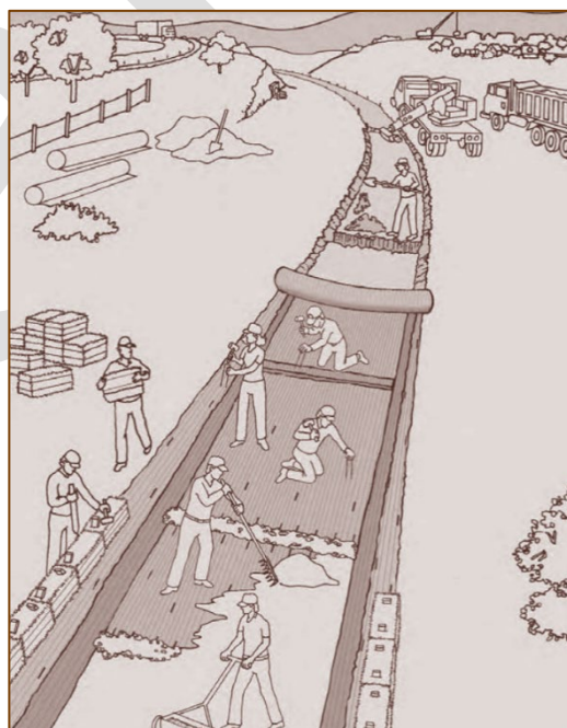
Figure 5- 14 Example of TRM Channel Application
