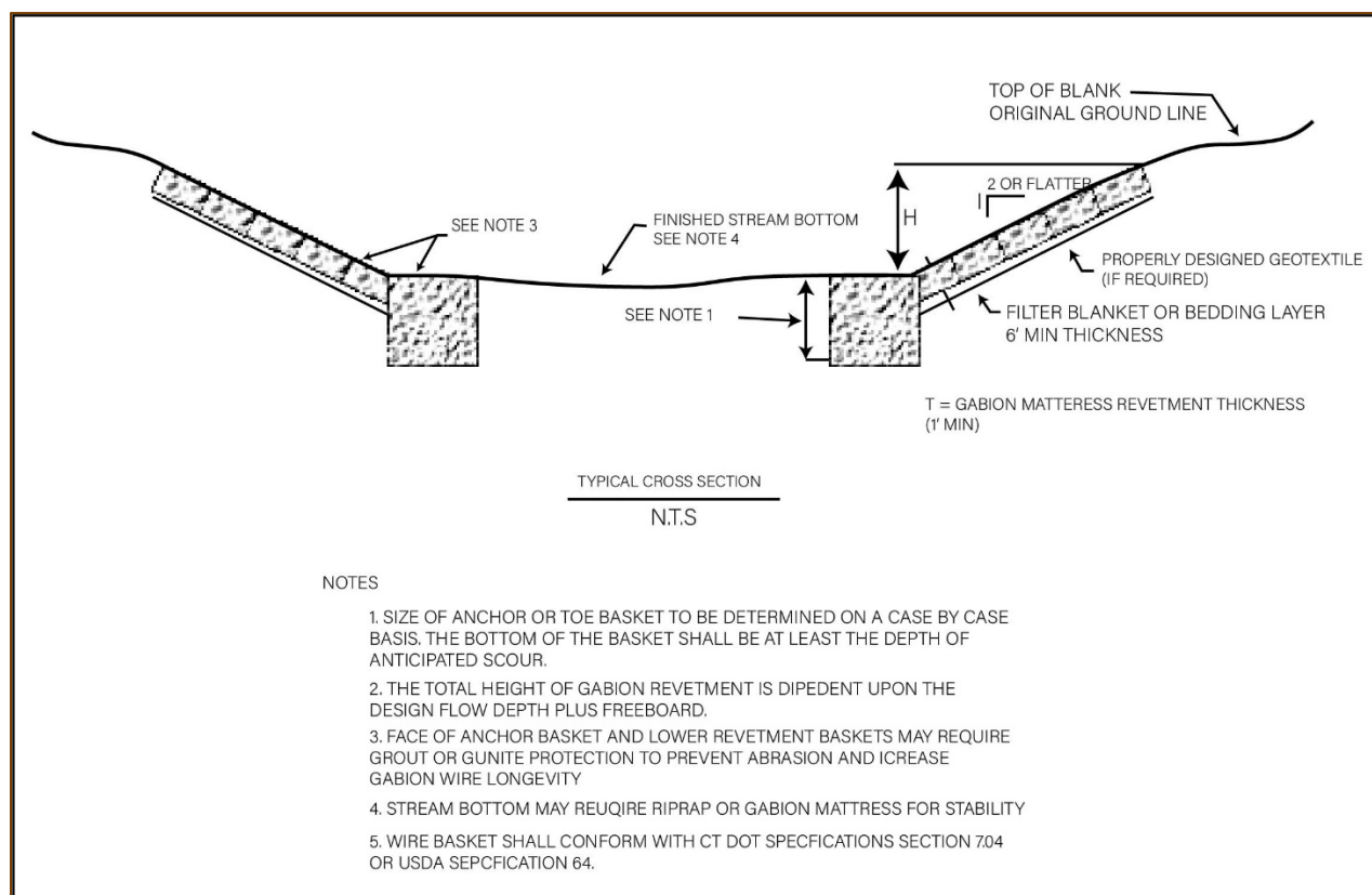
Figure 5- 23 Gabion Revetment
