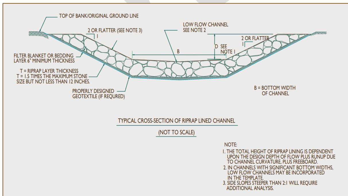
Figure 5- 21 Riprap for Armored Channel Stabilization
