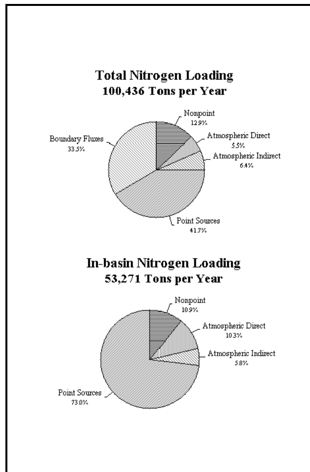
Figure 4. Sources of nitrogen to Long Island Sound.
