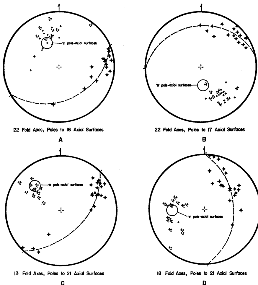
Fig. 15. Crenulate folds from Rattlesnake Hill, A , south to Taine Mountain, B , Barnes Hill, C , and Johnnycake Mountain northeastward to Burlington. Great circles that approximate the distribution of poles (dots with barbs) to axial surfaces are dashed. Symbol for fold axes is shown in figure 11.
