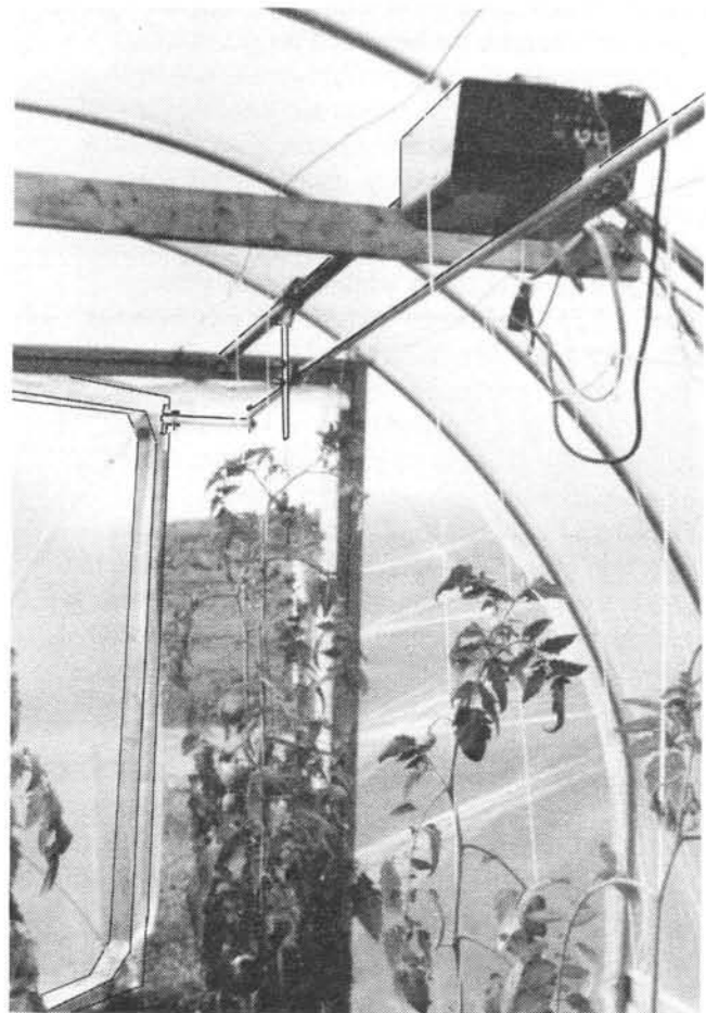
Figure 1. An interior view of the door of a high tunnel showing the method for automatic control of ventilation.
