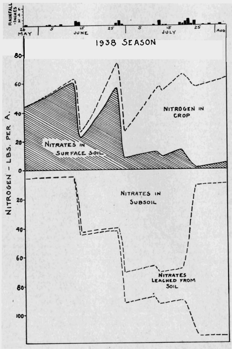
FIGURE 3. Distribution of nitrates during growing season of 1938.
