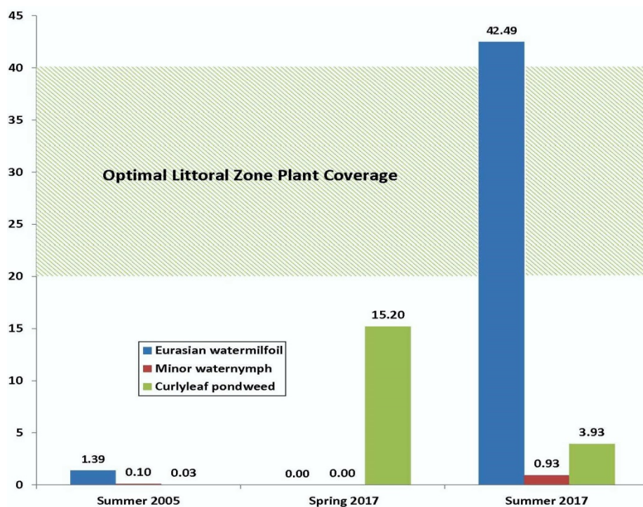
Figure 8. Littoral zone coverage of invasive aquatic plants in Lake Housatonic.
