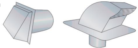
Wall and roof terminations for dryer exhaust must be undiminished in size and provide 12.5 square inches of area.
