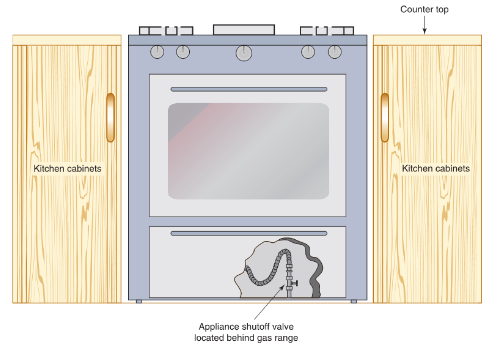
Shutoff valve behind gas range meets the requirement for access
