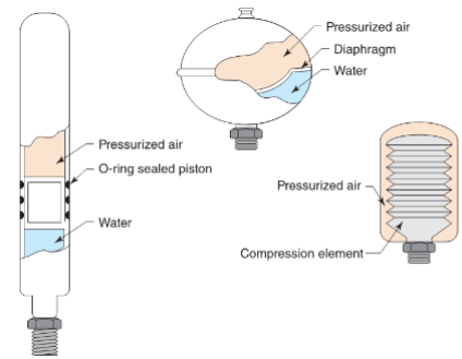
Examples of mechanical water hammer arrestors
