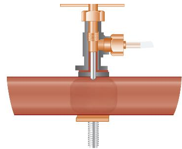
Saddle tap fitting
