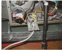
Photo 5. A gas furnace supplied by a branch circuit that has a metal gas piping system supplying it
