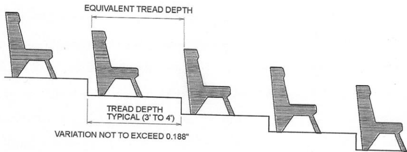
Figure 1029.13.2.1 TYPICAL SEATING PLATFORMS ALSO USED AS STEPPING AISLES
