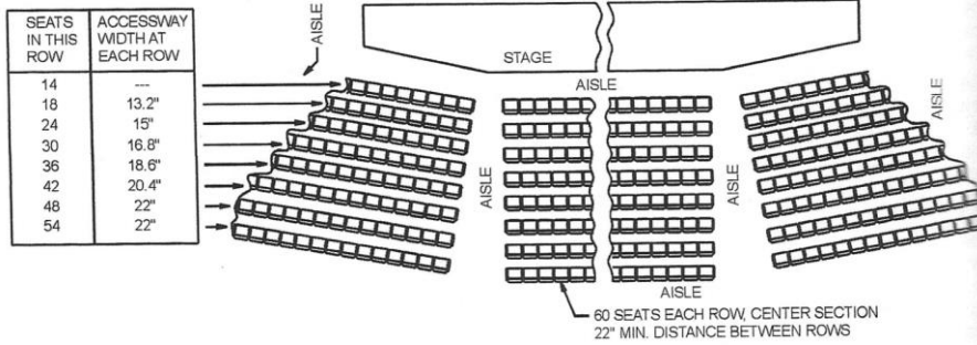
Figure 1029.12.2.1 TYPICAL DUAL-ACCESS ROW—MINIMUM AISLE ACCESSWAY WIDTH
