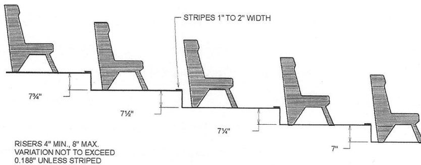
Figure 1029.13.2.2 TYPICAL RISER CONSTRUCTION IN STEPPED AISLES
