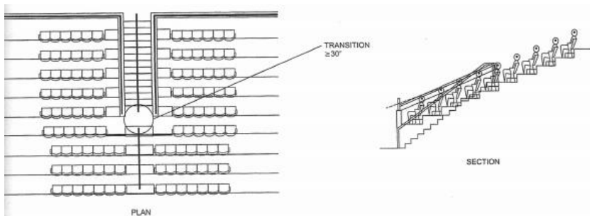
Figure 1029.10.2.1(2) TRANSITION BETWEEN STEPPED AISLE AND STAIRWAY AND THE LOWER END OF THE FLIGHT
