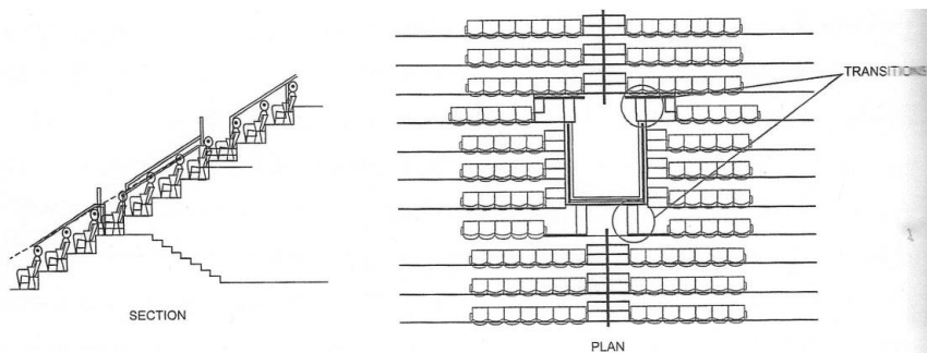
Figure 1029.10.2.2(2) EXAMPLE OF TURNS IN A STEPPED AISLE
