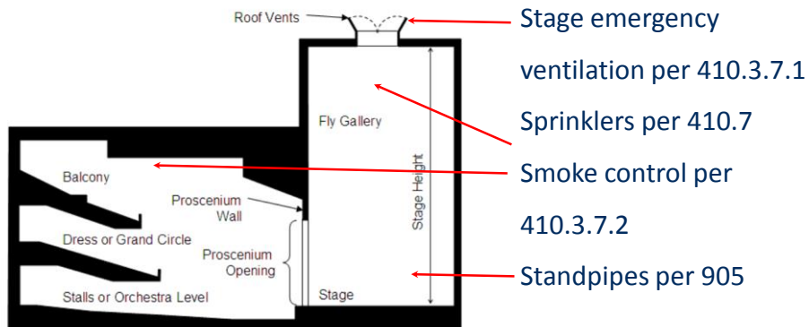
Figure 1 - Typical Theater Cross-Section
