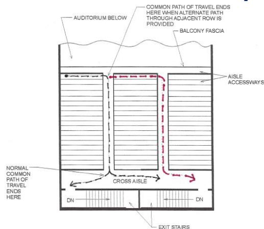
Figure 1029.8.1 PATH THROUGH ADJACENT ROWS
