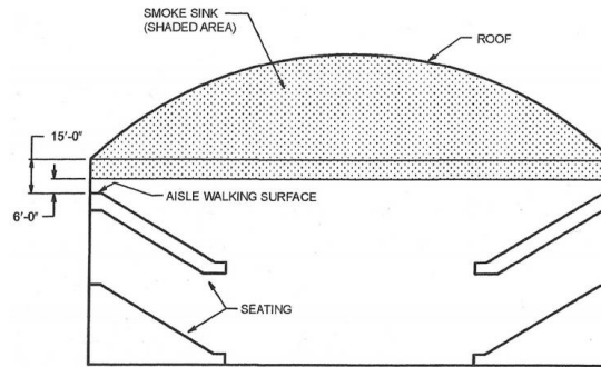
Figure 1029.6.2.2(1) ROOF HEIGHT (CONVEX DOME ROOF)
