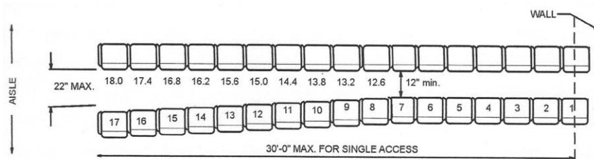
Figure 1029.12.2.2 TYPICAL SINGLE-ACCESS ROW—MINIMUM AISLE ACCESSWAY WIDTH FOR SEATS WITH BACKRESTS
