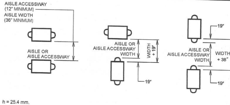
Figure 1029.12.1 AISLE AND AISLE ACCESSWAY MEASUREMENT WITH SEATING AND TABLES
