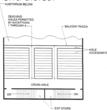
Figure 1029.9.5 TYPICAL BALCONY ARRANGEMENT
