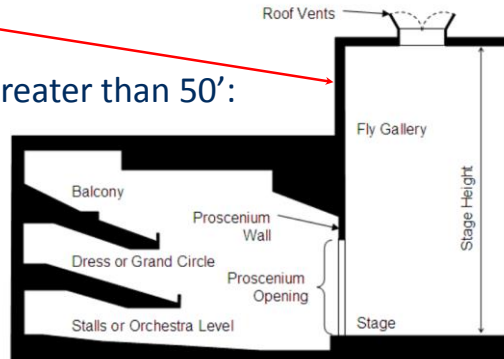
Figure 1 - Typical Theater Cross-Section
