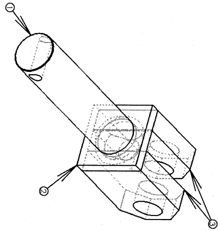
EYEBAR ASSEMBLY VIEW
