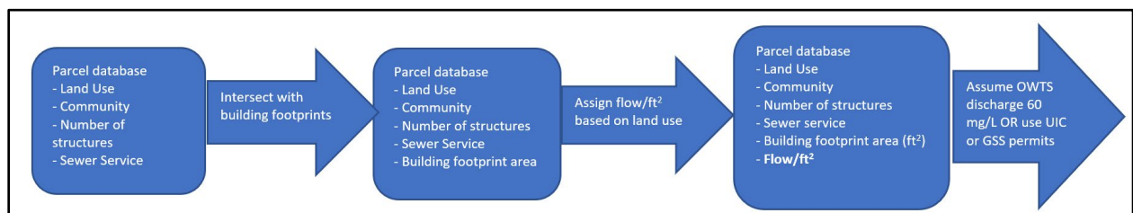
Figure 4b - Approach to Estimate Unattenuated Nitrogen Loads from Non-Residential Parcels
