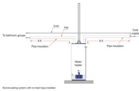
Noncirculating system with no heat traps installed
