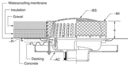
Specification cutaway view of a roof drain installation (Courtesy of Zum Industries, LLC)
