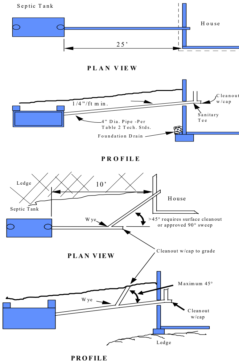
Figure 1 - Building Sewers
