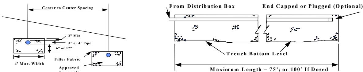
Figure 14 - Leaching Trenches
