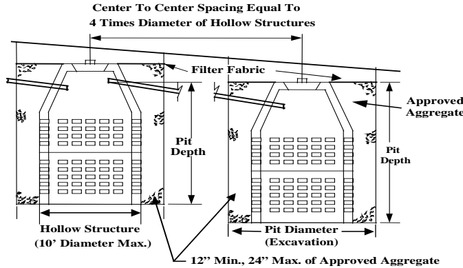
Figure 15 - Leaching Pits
