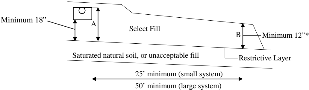
Diagram 6 – Select Fill Receiving Soil (Sloped Restrictive Layer)
