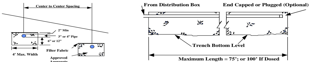
Figure 14 - Leaching Trenches
