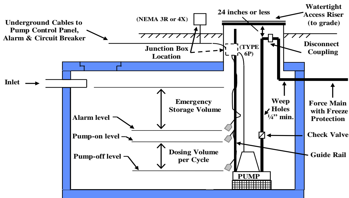
Figure 11 - Pump Chamber
