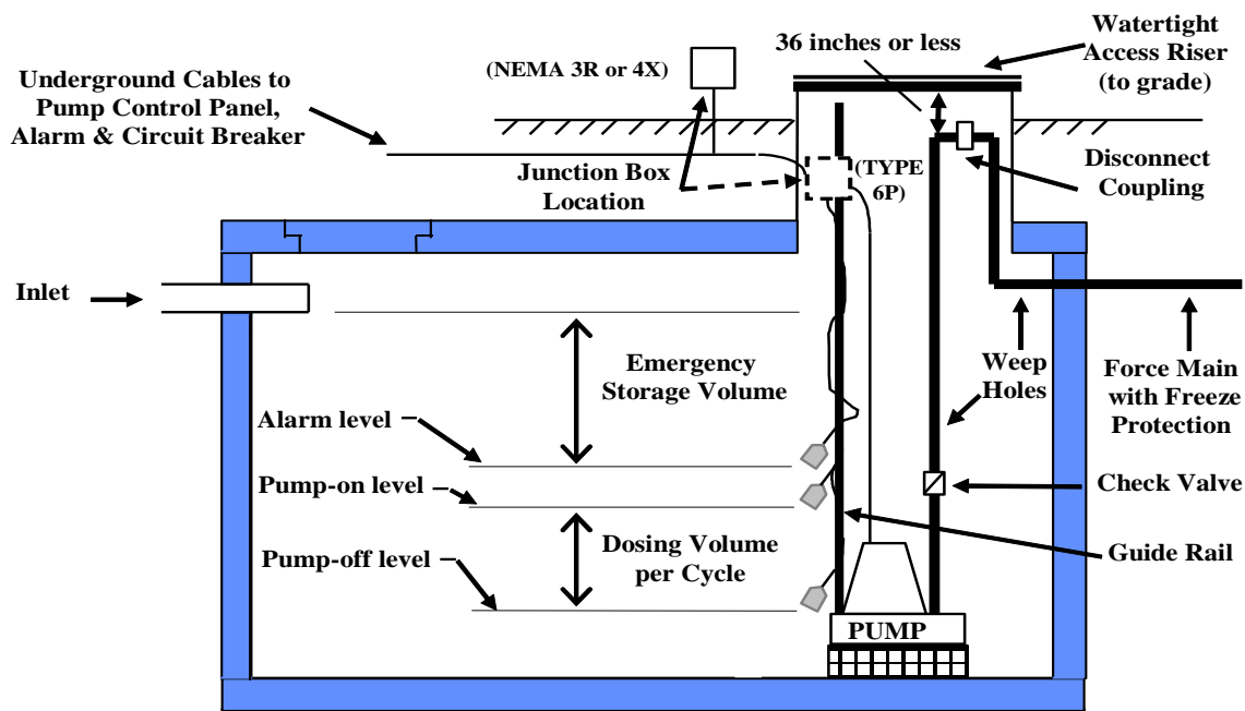
Figure 11 - Pump Chamber
