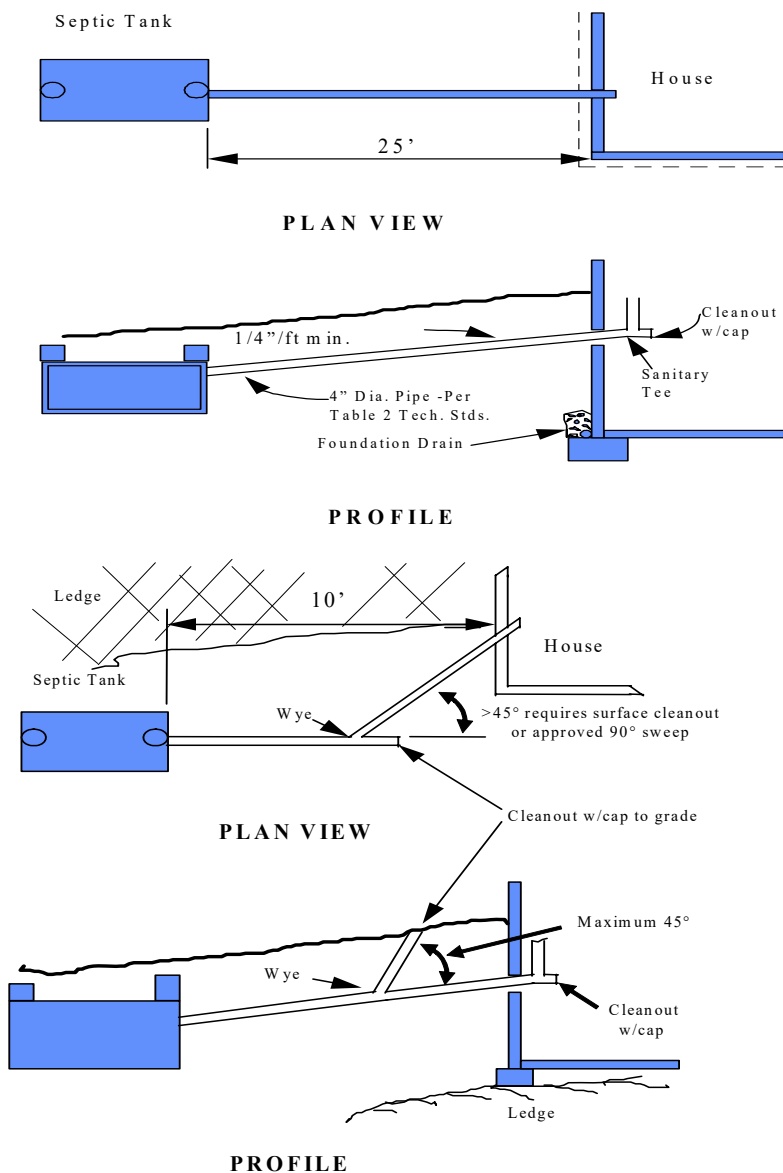
Figure 1 - Building Sewers
