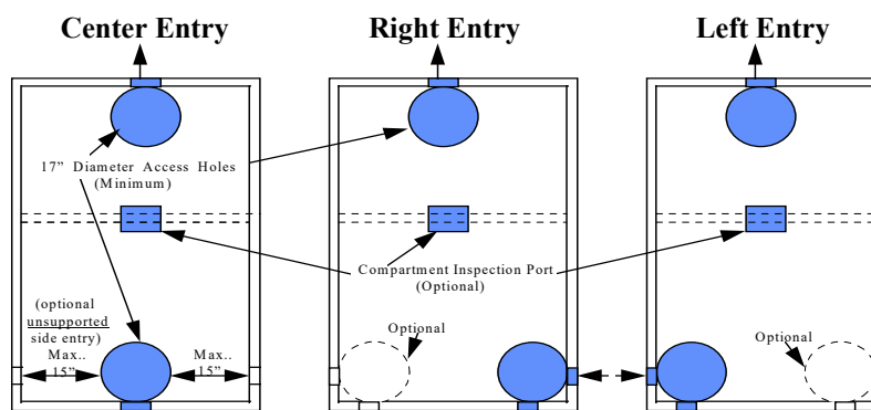
Figure 6 – Standard Septic Tank Configurations
