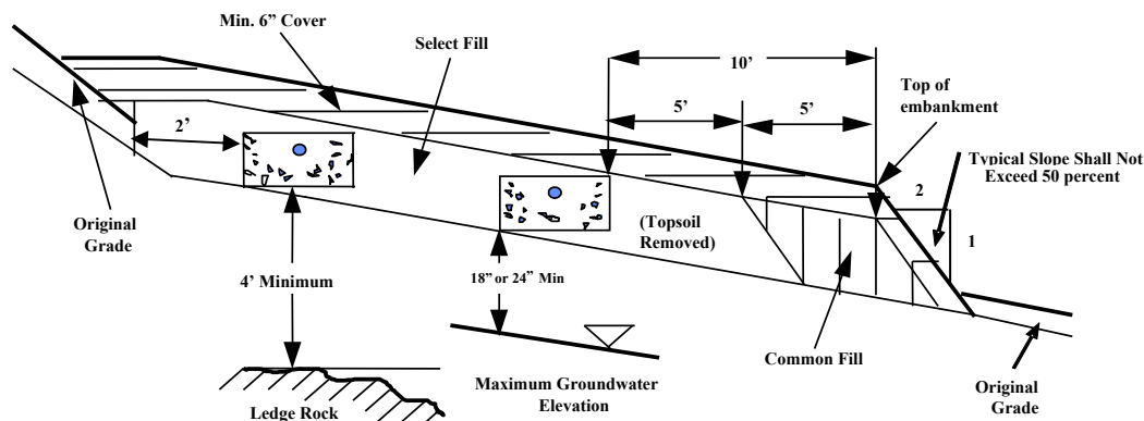
Figure 13 - Minimum Separating Distances above Ledge Rock and Maximum Groundwater
