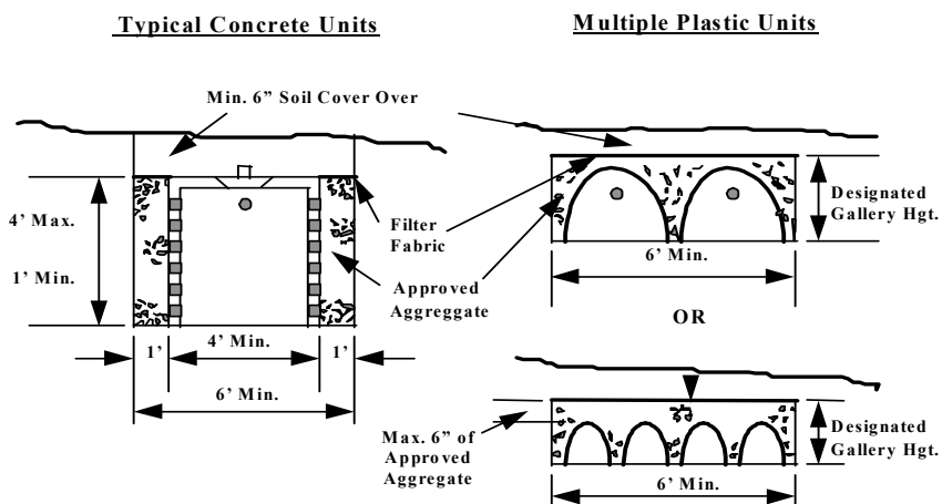
Figure 16 - Typical Leaching Gallery Structures
