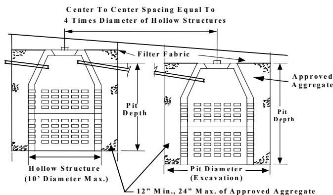
Figure 15 - Leaching Pits
