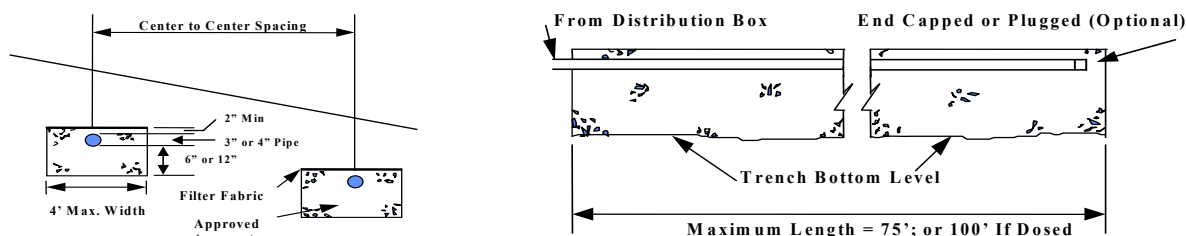
Figure 14 - Leaching Trenches
