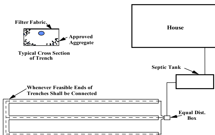
Figure 8 – Level Leaching Systems
