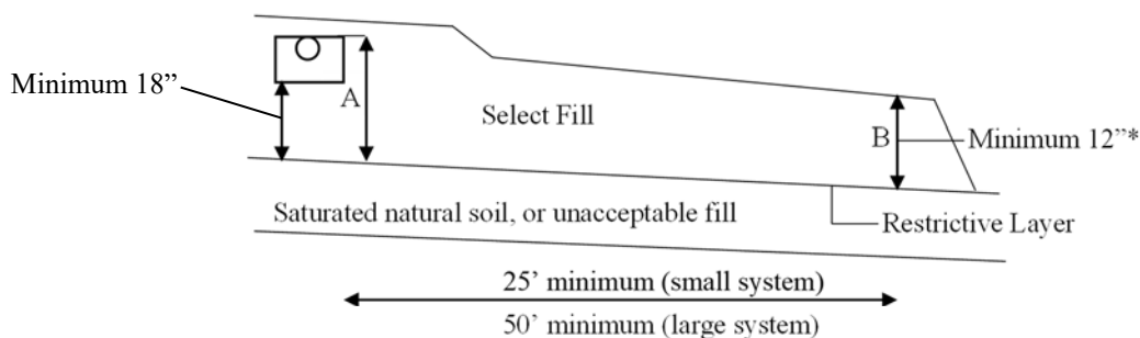
Diagram 6 – Select Fill Receiving Soil (Sloped Restrictive Layer)
