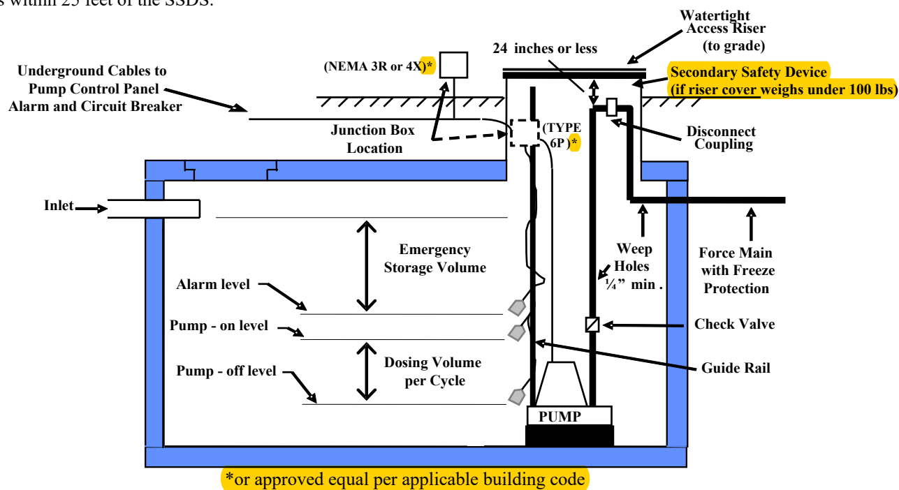
Figure 11 – Pump Chamber
