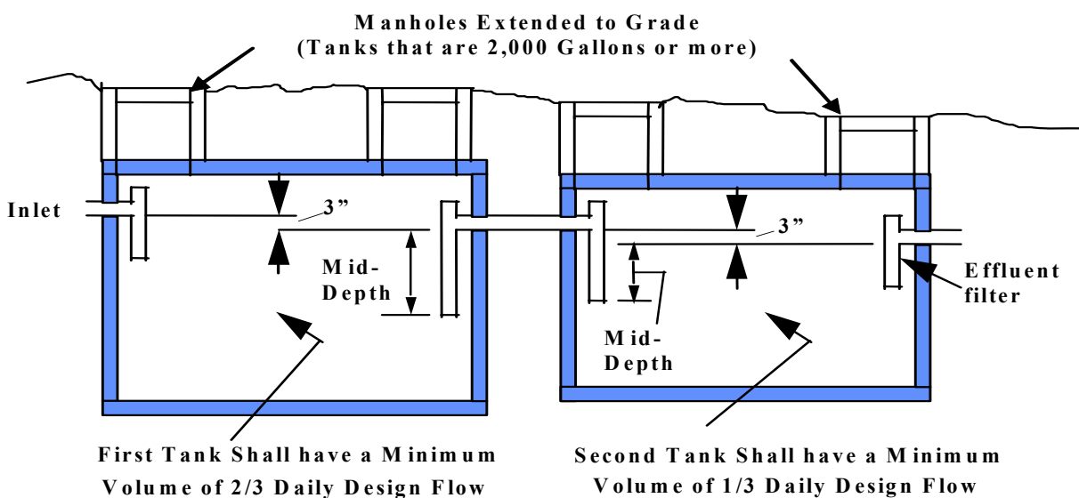
Figure 5 – Two Septic Tanks in Series
